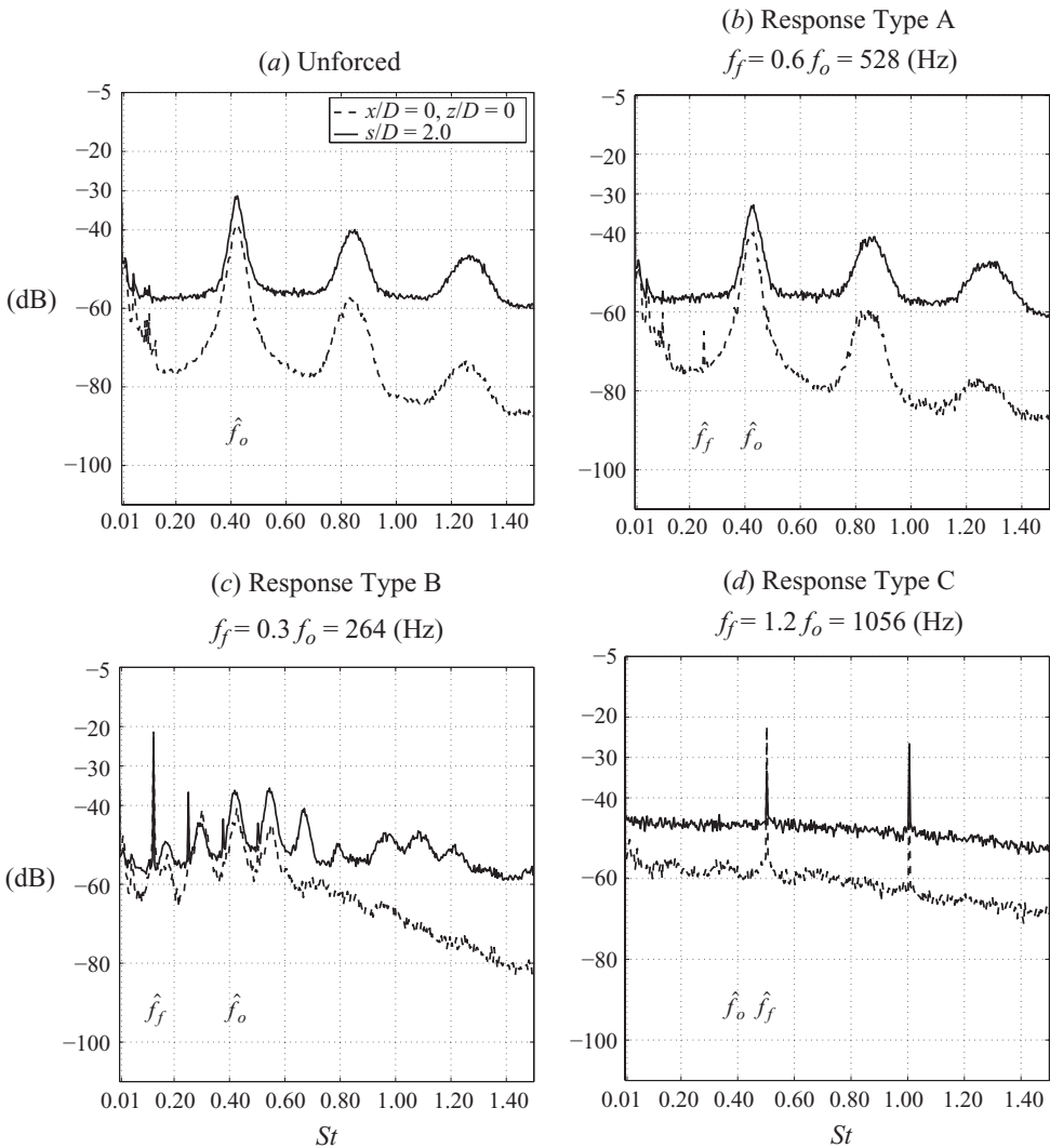
FIGURE 11. Upstream shear-layer spectra at R = 1.15 for: (a) no external forcing. (b) Excitation at frequency f_f = 0.6f_o and forcing amplitude equivalent to 1% of the mean jet velocity, an example where the peak at f_o was dominant. (c) Excitation at f_f = 0.3f_o and amplitude equivalent to 20% of the mean jet velocity, an example where the peak at f_o was present but not dominant. (d) Excitation at f_f = 1.2f_o and amplitude equivalent to 20% of the mean jet velocity, an example where the peak at f_o was invisible and that at f_f was dominant. Results in (b), (c) and (d) are typical of response types shown on the control map in figure 12(a).
