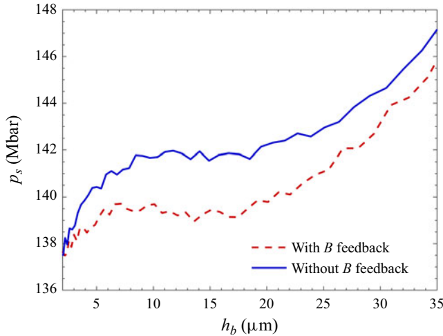
Figure 12. The pressure on the spike vertex p_s in the \lambda = 10 \mu\text{m} case without (case ii) and with (case xv) magnetic feedback.
