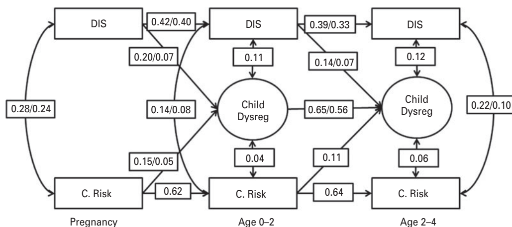
Fig. 2. Multiple group path analysis. Path coefficients: depressed/non-depressed or averaged across all mothers; single arrow paths = predictions; double arrow paths = correlations; circles = latent variables (items not shown for the sake of a simple presentation); rectangular = manifest variable. All parameters shown are significant at p < 0.05 . The pathways from child emotional and behavioral dysregulation (Child Dysreg) to dependent interpersonal stress (DIS) and contextual risks (C. Risk) failed to reach significance; predictions between DIS and C. Risk are not shown for the simplicity of the presentation (and because these relationships are not central to the current research questions), but are available on request from the author.
