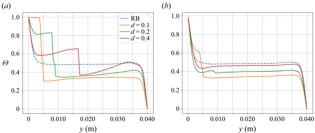
Figure 19. Time-averaged vertical profiles of non-dimensional temperature \theta = (T - T_c)/\Delta T at (a) x = 0.5L_1 and at (b) x = 0.2L_1 for \Gamma_1 = 4.25 , \Gamma_2 = 1.73 and Ra = 8.6 \times 10^6 .
