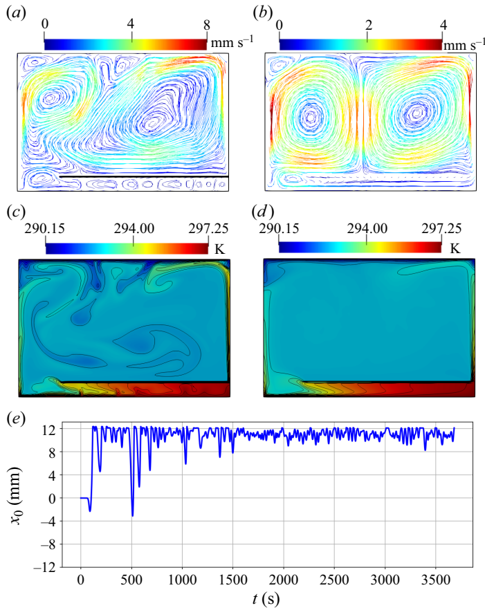
Figure 10. Distributions of (a,b) velocity and (c,d) temperature for \Gamma_1 = 1.53 , \Gamma_2 = 1.25 , Ra = 8.6 \times 10^6 and d = 0.1 . (a,c) Instantaneous and (b,d) average fields are shown. Panel (e) presents the displacements of the plate. (Numerical simulations.)
