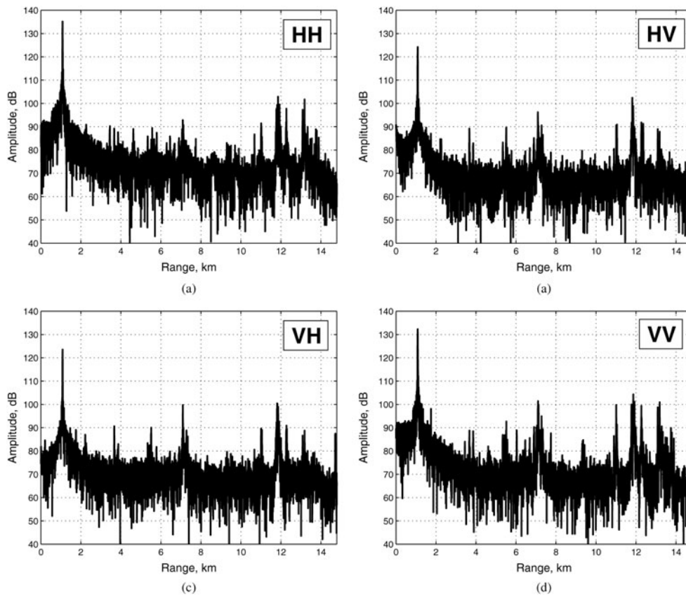
Fig. 10. PARSAX radar range profiles in case of simultaneous sounding with two orthogonal LFM waveforms and cross-channel interferences suppression.
