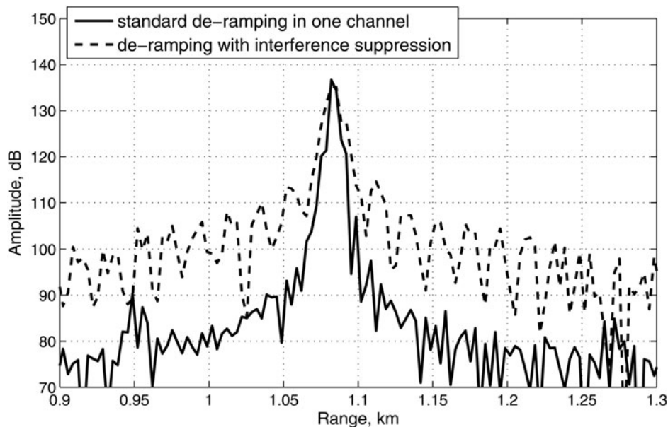
Fig. 11. Zoomed part of the HH amplitude profiles, which were measured by the PARSAX radar in cases of one-waveform sequential polarimetric measurements (solid line) and simultaneous sounding with two orthogonal LFM waveforms and cross-channel interferences suppression (dashed line).
