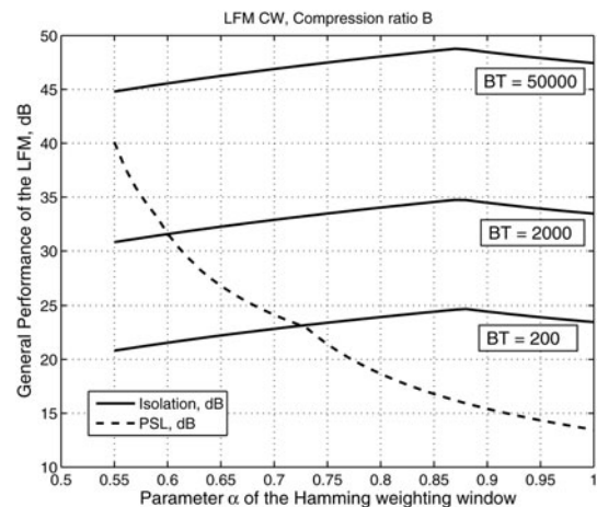
Fig. 3. Performance parameters of the FM-CW polarimetric radar with dual-orthogonal LFM signals.
