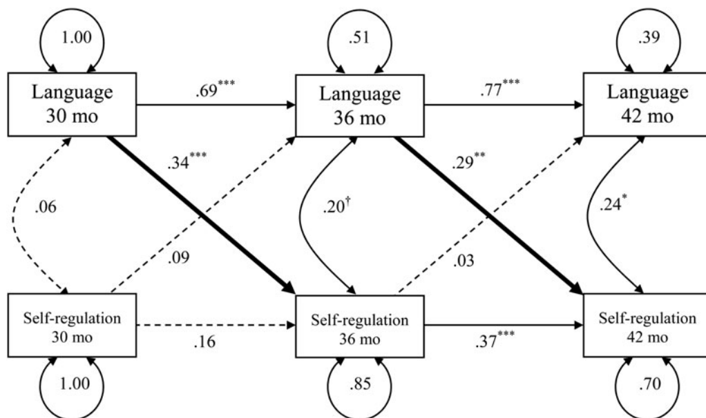
Figure 1. Cross-lagged model with language ability and self-regulation, as measured by the bird/alligator task. Estimates represent standardized regression coefficients. Bold lines represent significant cross-lagged paths. Dashed lines represent nonsignificant paths. † p < .10 , * p < .05 , ** p < .01 , *** p < .001 .
