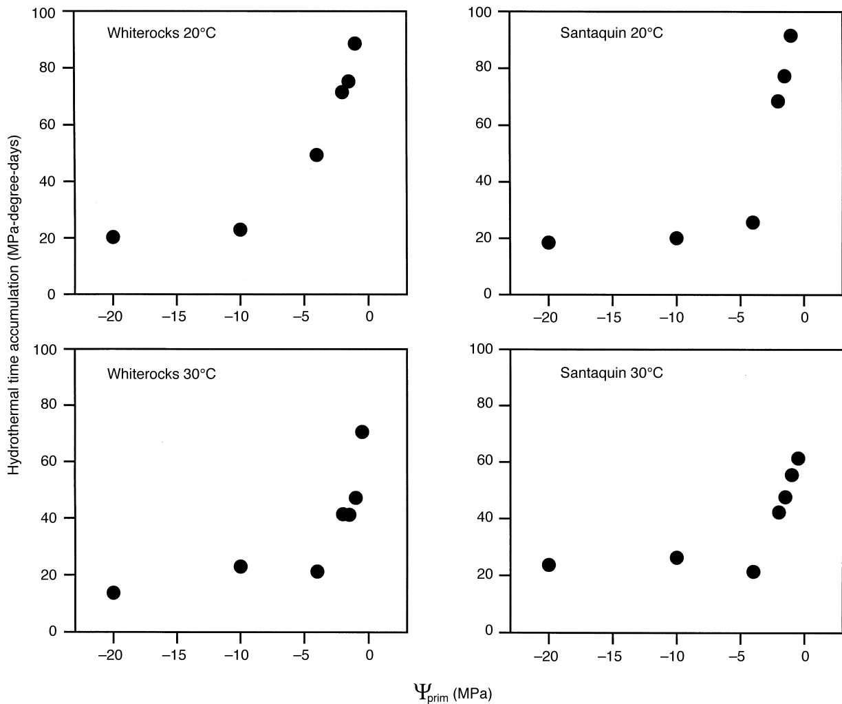
Figure 3. Hydrothermal time accumulation during a week of priming plotted as a function of priming water potential for fully after-ripened seeds from two populations of Elymus elymoides primed and incubated at two temperatures.
