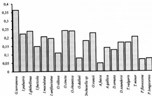
Fig. 5. Comparison of average heterozygosity estimates (He) of G. terranova with those obtained in other collembolan species. Data for other species are from: Carapelli et al. (1997) ( Isotomurus palustris (Müller, 1776), I. ghibellinus (Carapelli et al. , 1995), I. fucicola (Reuter, 1891), I. maculatus , I. unifasciatus (Schäffer, 1896)); Frati et al. (1994) ( Orchesella villosa , O. cincta (Linné, 1758), O. chianica (Frati and Szeptycki, 1990), O. dallaii (Frati and Szeptycki, 1990), Orchesella sp. , O. ranzii (Parisi, 1960)); Fanciulli et al. (1994) ( Allacma fusca (Linné, 1758), A. gallica ); Fanciulli et al. (1995) ( Dicyrtomina ornata , D. saundersi (Lubbock, 1862)); Fanciulli et al. (2000) ( Tomocerus vulgaris , T. minor (Lubbock, 1862), Pogonognathellus flavescens , P. longicornis (Müller, 1776)).
