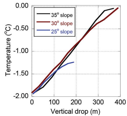
Fig. 6. Temperature calculations performed on the inclined plane with identical mass and initial temperature, but with three different slope angles ( 25^\circ, 30^\circ, 35^\circ ) and no entrained mass. Note that temperature gradient with vertical drop is the same for the three cases. However, the example calculated with 25^\circ stopped before reaching 0^\circ\text{C} , whereas the other two cases reached 0^\circ\text{C} after dissipating the same amount of potential energy ( \sim 380 m vertical).
