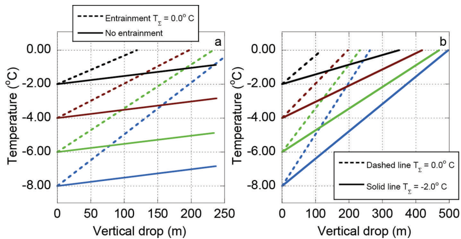
Fig. 7. Temperature calculations performed on the inclined plane with identical slope angle, 35^\circ , and identical initial mass, but varying the temperature of the released mass. (a) Different release temperatures from -2 to -8^\circ\text{C} entraining snow at 0.0^\circ\text{C} (dashed line) and with no entrainment (solid line). Note that with no entrainment the avalanche stops before reaching 0^\circ\text{C} , but with entraining snow at 0^\circ\text{C} the avalanches reached the melting point after different vertical drops, depending on the initial temperature. (b) Different release temperatures from -2 to -8^\circ\text{C} entraining snow at 0^\circ\text{C} (dashed line) and -2^\circ\text{C} (solid line). The varying slopes of the lines are the result of the relative temperature differences between released and entrained snow.
