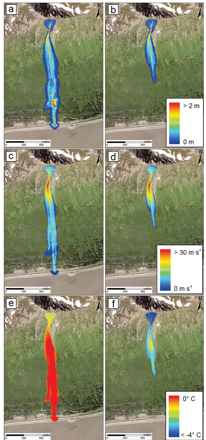
Fig. 16. Avalanche calculations at Whiskey no. 934, Bird Hill. Release is situated at 1000 m a.s.l. and finishes on the coastline. The left column (a, c, e) shows the flow height, velocity and temperature calculations for an example calculated with T_0 = -2^\circ\text{C} and T_\Sigma = -1^\circ\text{C} . The right column (b, d, f) shows the same calculations, but modifying the release temperature and the entrainment temperature to T_0 = -4^\circ\text{C} and T_\Sigma = -4^\circ\text{C} . Note the difference in runout distance and velocity between both simulations after modifying the initial temperature conditions.
