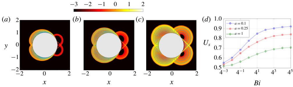
FIGURE 12. Force-free squirmer solutions showing \log_{10} \dot{\gamma} for the normal surface velocity condition (2.11) with (a) a=0.1 , (b) 0.25 and (c) 1 , at Bi=2^8 . (d) The variation of the swimming speed with Bi .
