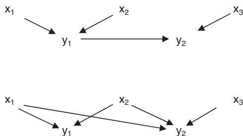
FIGURE 1. Upper panel: y_1 causes y_2 . Lower panel: y_1 does not cause y_2 due to failure of the sufficiency condition
