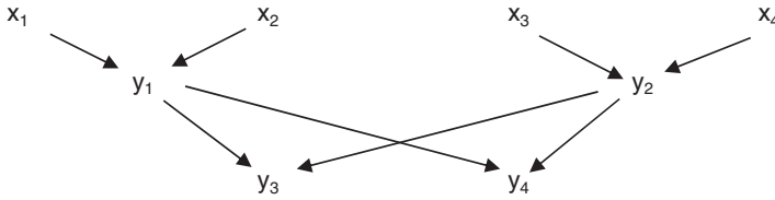
FIGURE 2. Paths connecting y_1 and y_2 are blocked by colliders y_3 and y_4
