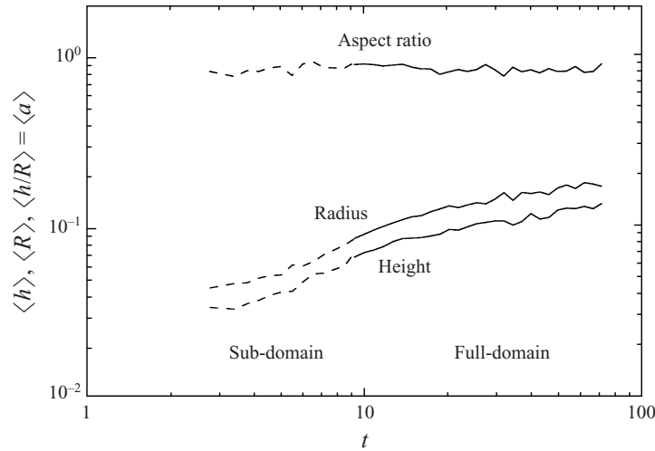
FIGURE 8. The population-mean vortex-element radius, \langle R \rangle(t) , half-height, \langle h \rangle(t) , and aspect ratio, \langle a \rangle(t) , from the vortex census.
