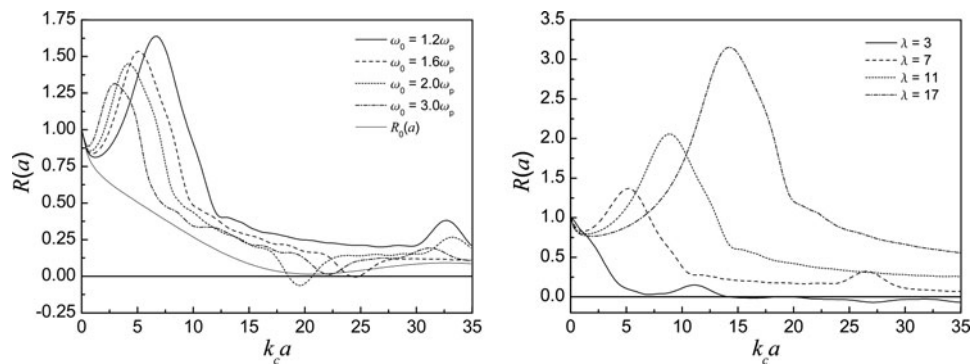
Fig. 2. (Left panel) the ratio R(a) = S(a)/S_B as a function of dimensionless quantity k_c a at v = 8.6v_c , \omega_0 = 1.2\omega_p (solid line), \omega_0 = 1.6\omega_p (dashed line), \omega_0 = 2\omega_p (dotted line), \omega_0 = 3\omega_p (dash-dotted line). Thin solid line corresponds to R_0(a) = S_0(a)/S_B (see Eq. (33)). (Right panel) same as in left panel but at \omega_0 = 1.2\omega_p , v = 3v_c (solid line), v = 7v_c (dashed line), v = 11v_c (dotted line), v = 17v_c (dash-dotted line).
