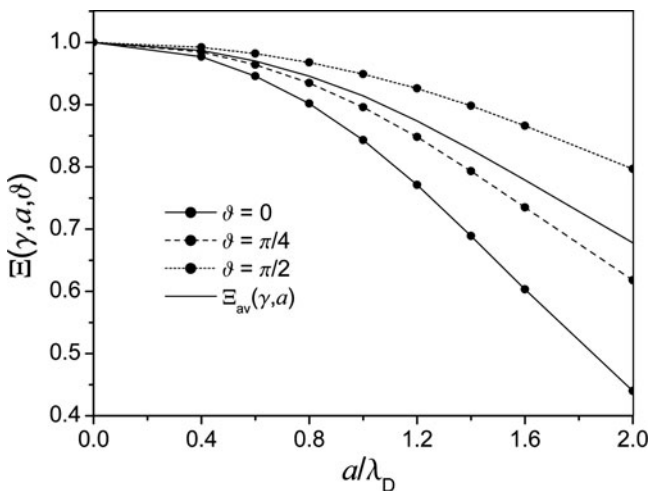
Fig. 1. The dimensionless quantities \Xi(\gamma, a, \vartheta) (the lines with symbols) and \Xi_{av}(\gamma, a) (the solid line without symbols) vs the intensity parameter of the laser field a/\lambda_D for \vartheta = 0 (solid line), \vartheta = \pi/4 (dashed line), \vartheta = \pi/2 (dotted line) and for \omega_0 = 1.2\omega_p .
