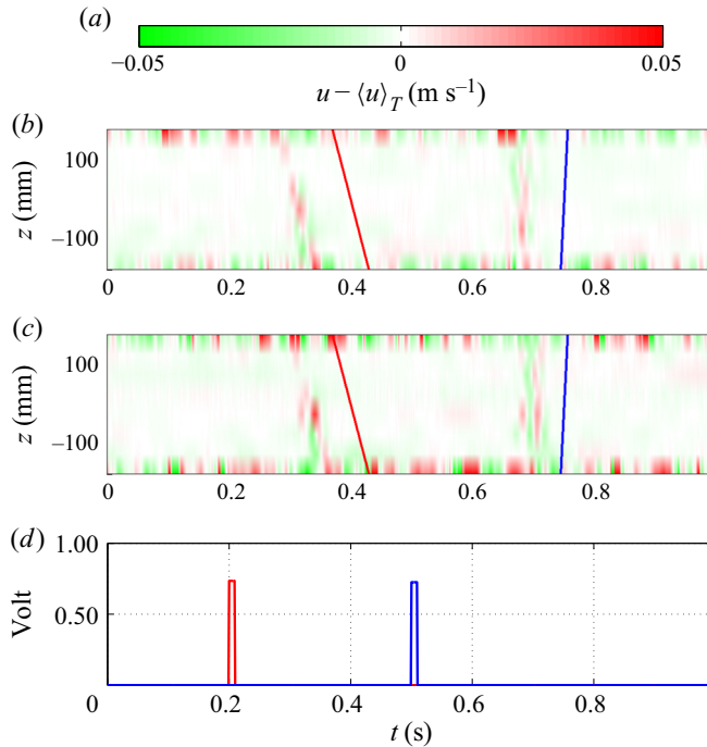
Figure 24. Time histories of streamwise disturbance velocity at two downstream stations. (a) Colourbar for (b,c). Time history of streamwise disturbance velocity at (b) y = 0.9 mm, x = 600 mm and (c) y = 0.9 mm, x = 650 mm. (d) Pulsation sequence of actuator parallel to leading edge (blue) and inclined actuator (red). Free-stream velocity is U = 5 m s -1 . In (b,c) the estimated values of WP envelope inclination angles are denoted by the red ( s_2 ) and blue ( s_1 ) lines.
