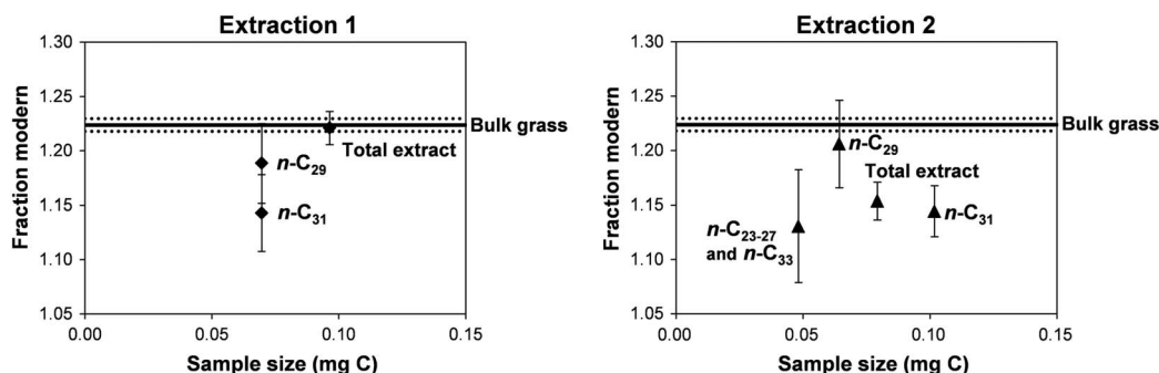
Figure 3 Fraction modern ( F^{14}\text{C} ) values of grass n -alkanes PCGC-isolated from two independent extraction methods. Also shown are the F^{14}\text{C} values of the total n -alkane fraction (“Total extract”; before PCGC isolation of individual n -alkanes) from each method. The F^{14}\text{C} value of the grass (bulk combusted; n = 11 ) and standard deviation are shown as solid and dotted lines, respectively.
