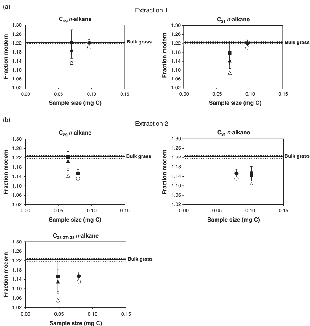
Figure 4 Fraction modern ( F^{14}\text{C} ) values of n -alkanes (triangles and squares) and total n -alkane extract (circles) from (a) extraction 1 and (b) extraction 2. F^{14}\text{C} values before and after correction for extraneous carbon ( \text{C}_{\text{ex}} ) added during sample preparation are shown as open and closed symbols, respectively. Correction for \text{C}_{\text{ex}} added during PCGC isolation and solvent removal (excludes chemical extraction, Table 1) is shown in triangles and correction for \text{C}_{\text{ex}} added during the entire sample procedure (chemical extraction + PCGC + solvent removal, based on \text{C}_{29} n -alkane isolated from the grass, Table 3) is shown in squares. The total n -alkane extract was corrected for \text{C}_{\text{ex}} derived from solvent removal. The F^{14}\text{C} value of the grass (bulk combusted; n = 11 ) and standard deviation are shown as solid and dotted lines, respectively.
