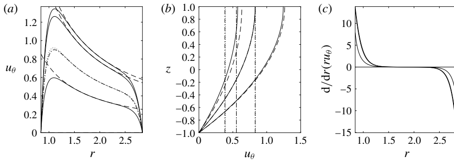
FIGURE 5. (a,b) The quasi-two-dimensional azimuthal velocity profiles and (c) the Rayleigh criterion for inviscid centrifugal instability for an electrolyte layer placed in a uniform vertical magnetic field at \epsilon = 0.083 , Ha = 1.69 \times 10^{-3} , Re = 1.1 \times 10^2 and Fr^2 = 4.4 \times 10^{-3} (corresponding to B_0 = B_z = 0.02 T, I_0 = 0.05 A and h = 2.5 mm). The profiles are shown for z = 1.0, 0.5 and -0.5 in panels (a) (top to bottom) and (c), and for r = 1.30, 1.98 and 2.60 (right to left) in panel (b). The solid and dashed lines represent the numerical and exact solutions (5.9) respectively. The dash-dotted and dotted lines show the depth-averaged profiles obtained from (5.7) and (5.19) respectively.
