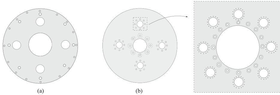
FIGURE 1. Panels (a) and (b) illustrate the concept of infinite outer-connectivity and infinite inner-connectivity, respectively. Panels (a) and (b) also accurately describe the topology of the m.c.w.d.s in [Bis18] and Theorem 1.1, respectively. As seen, the structure in panel (b) is more intricate.
