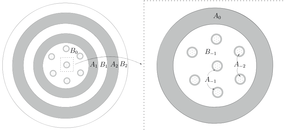
FIGURE 8. Illustration of Definition 7.1 of A_k, B_k for negative k . Each connected component of A_0 maps conformally onto A_1 ; therefore, each connected component of A_0 contains 2^N many connected components of A_{-1} . The picture repeats itself as we zoom in. The set B_0 is the region between the outer boundaries of the components of A_0 and the inner boundary of A_1 .
