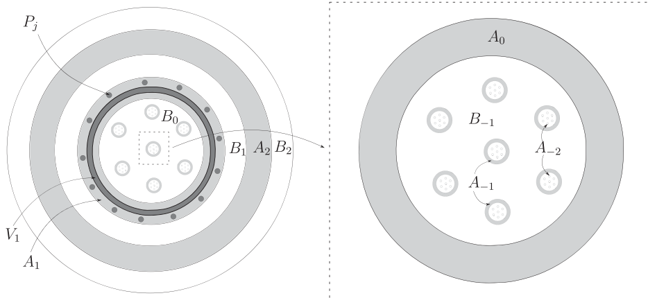
FIGURE 2. Definition of A_k, B_k for all k \in \mathbb{Z} . The annuli A_k are shaded light gray and the B_k are white. Also shown are V_1 \subset A_1 and the ‘petals’ P_j \subset A_1 (in dark gray).
