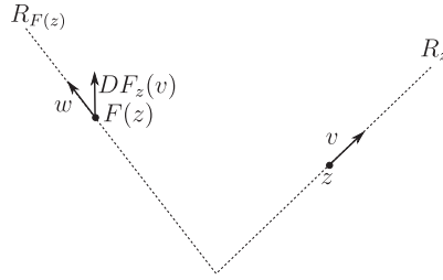
FIGURE 11. A schematic for the statement of Lemma 9.3.
