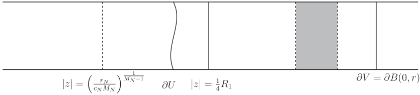
FIGURE 5. A schematic for Definition 5.4 and Lemma 5.5. The critical points for q_N lie on the circle |z| = (r_N/c_N M_N)^{1/M_N-1} , and the associated critical values lie in an annulus contained in V , illustrated in gray. So, U contains the critical points of q_N , and it will also be verified that U \subset D .
