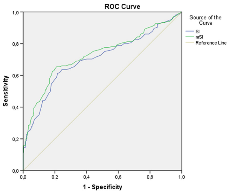
Figure 2. The ROC curves of SI and mSI for ICU admissions.
