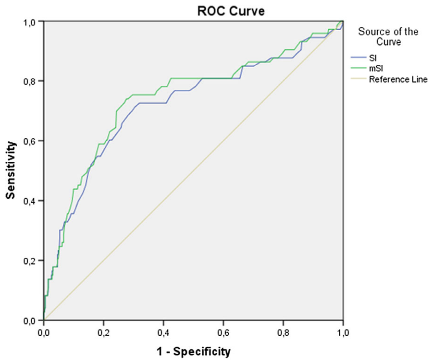
Figure 1. The ROC curves of SI and mSI for in-hospital mortality.
