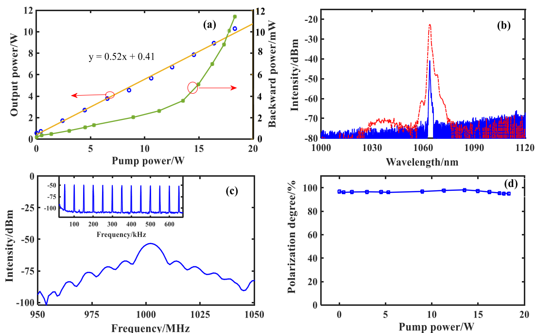
Figure 5. Output characterizations. (a) The output power and backward power versus pump power. (b) The output spectrum of injected seed and maximum output. (c) The RF spectrum. (d) The polarization degree versus different pump power.
