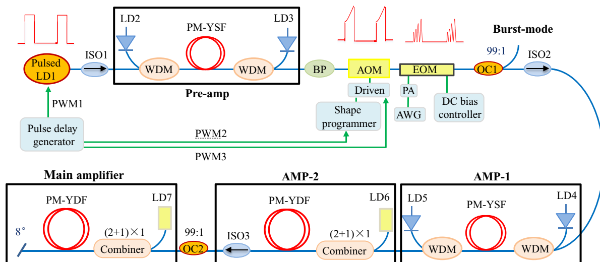
Figure 1. Schema of the linear-polarization burst-mode all-fibre laser system.
