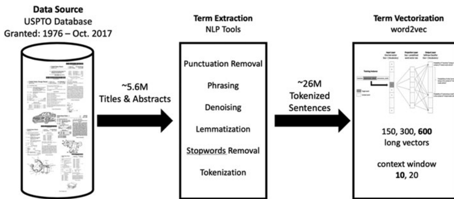
Fig. 1. A summary of the TechNet construction process (Sarica et al., 2020).
