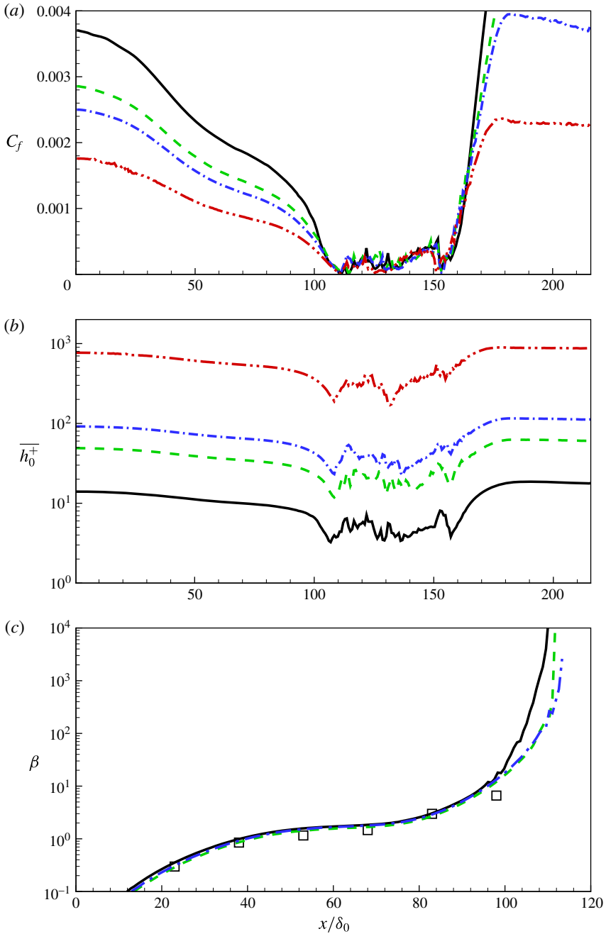
FIGURE 17. (Colour online) Effect of Reynolds number: —, Re_\theta^{in} = 2000 ; ----, Re_\theta^{in} = 8000 ; - · - ·, Re_\theta^{in} = 16\,000 ; - · · - ·, Re_\theta^{in} = 10^5 ; □, from experimental data of Perry & Fairlie (1975). (a) C_f versus x/\delta_0 ; (b) \overline{h_0^+} versus x/\delta_0 ; (c) \beta versus x/\delta_0 .
