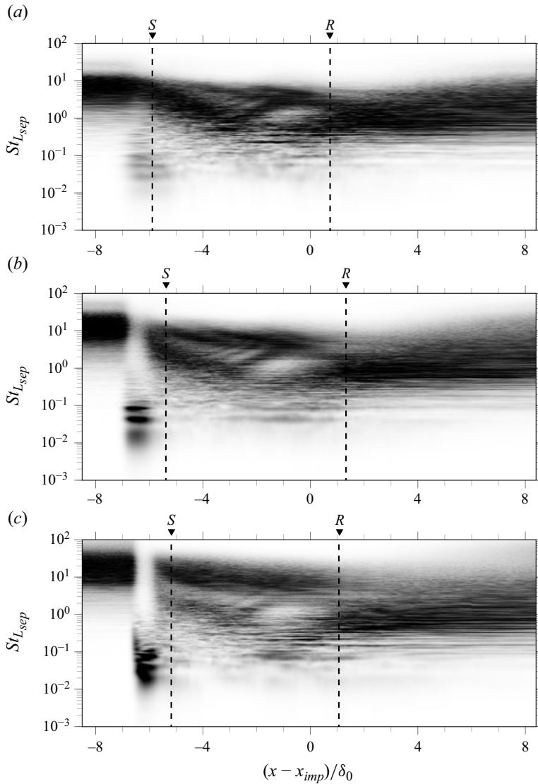
Figure 16. Frequency-weighted and normalized PSD map of wall pressure at the centreline: (a) case \mathcal{B}_1 ; (b) case \mathcal{B}_2 ; (c) case \mathcal{B}_3 . Dashed lines indicate mean separation ( S ) and reattachment ( R ) locations for each case. Contour levels range from zero (white) to 0.3 (black).
