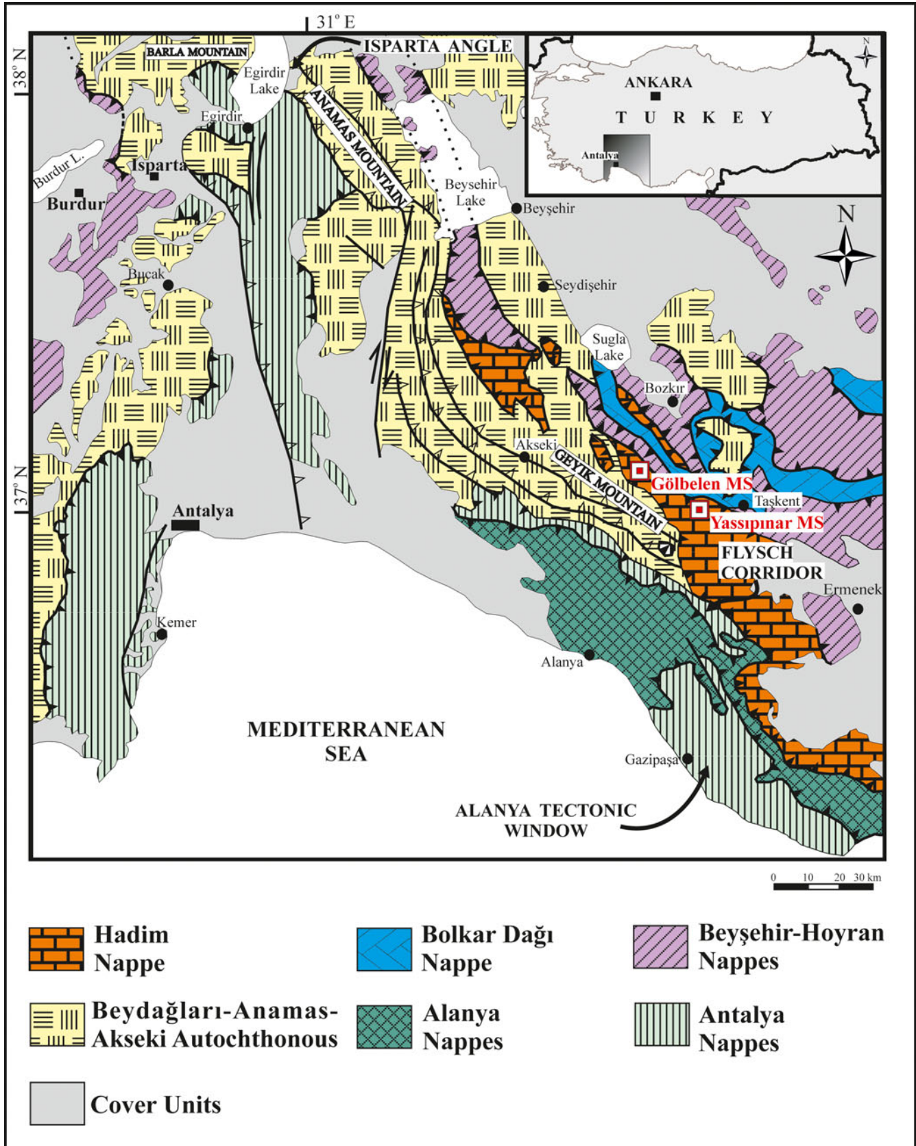
Figure 1. Schematic map showing the distribution of autochthonous and allochthonous sequences in the area between the Western and Central Taurides with the location of the Yassıınar and Gölbelen measured sections (MS) (simplified and revised after Özgül, 1984).
