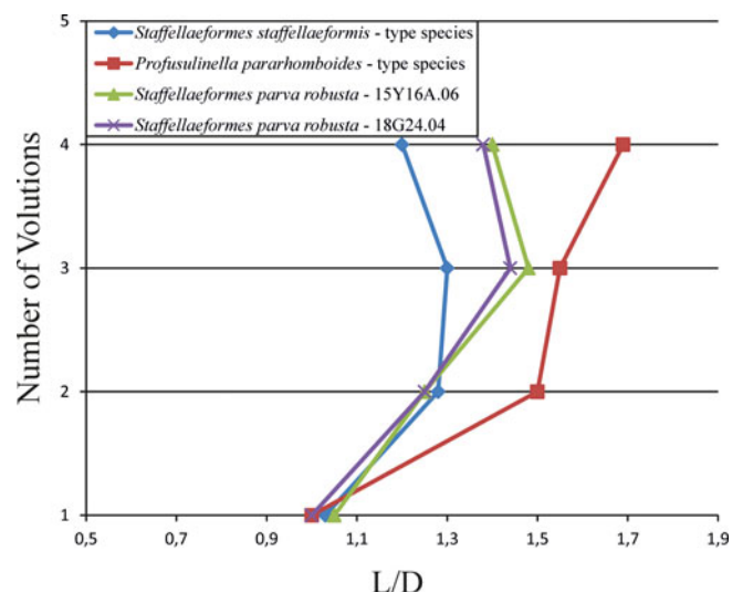
Figure 13. L/D Correlation graph between the type species of the Staffellaeformes and Profusulinella , and L/D ratio of Staffellaeformes parva robusta n. comb.
