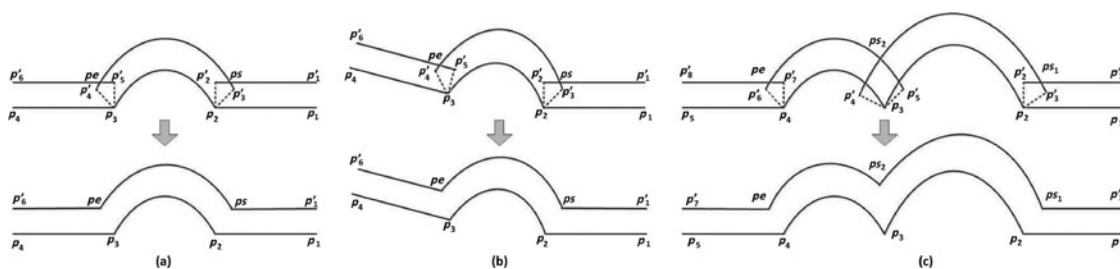
Fig. 8. Removing local invalid loops for arc offsets: (a) Arc within a same line, (b) arc with different lines at its two ends and (c) two consecutive arcs in the main polygon.
