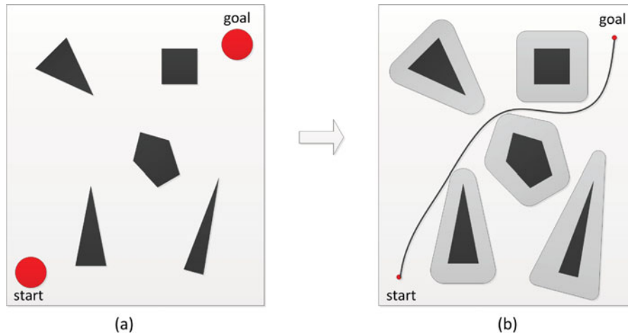
Fig. 1. Polygon offsetting in robot motion planning: (a) Workspace of a circular robot with polygonal obstacles and (b) configuration space of the robot after offsetting the workspace obstacles. A circular robot in the workspace is represented by a point in the configuration space. A sample path is also shown from the start to the goal position.
