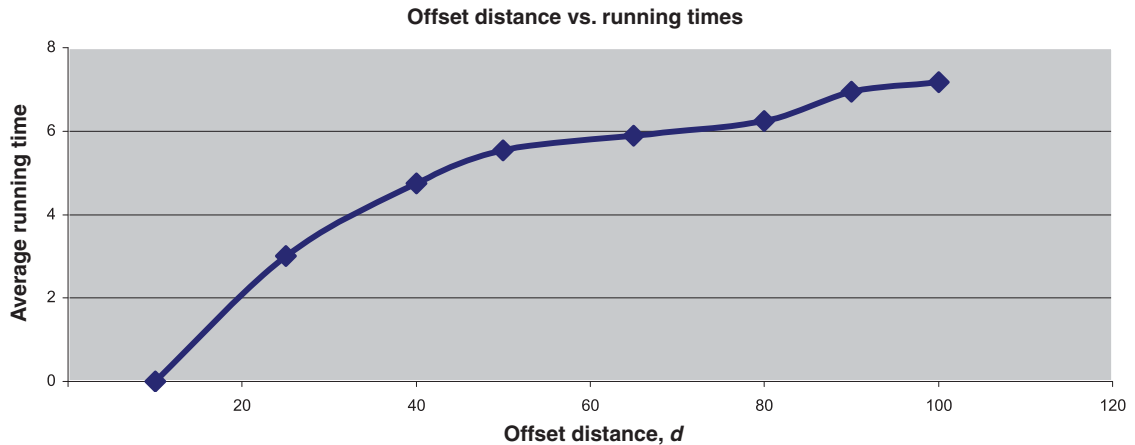
Fig. 16. Plotted result of Table II. Effect of offset distance on the comb output.
