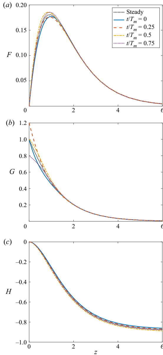
Figure 2. Velocity profiles (a) F , (b) G and (c) H , as functions of the wall-normal z -direction, for Reynolds number Re = 500 , modulation amplitude \epsilon = 0.2 and frequency \varphi = 8 . Results are plotted at t/T_m = 0 (blue solid lines), t/T_m = 0.25 (red dashed), t/T_m = 0.5 (yellow dot-dashed) and t/T_m = 0.75 (purple dotted). The steady solution is given by the black dotted lines, while T_m denotes one full cycle of disk modulation.
