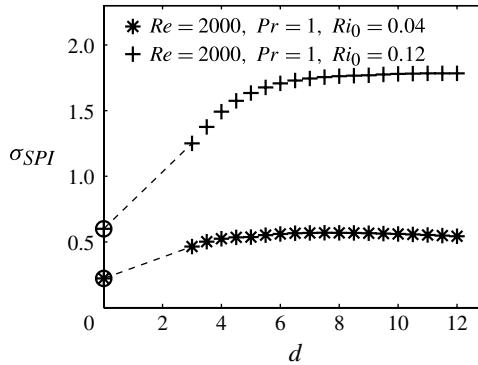
FIGURE 13. Growth rate versus spanwise wavenumber curves for two cases at a Re = 2000 . Both cases include d = 0 data points (encircled) and suggest that the growth rate curves should extend to d = 0 in principle.
