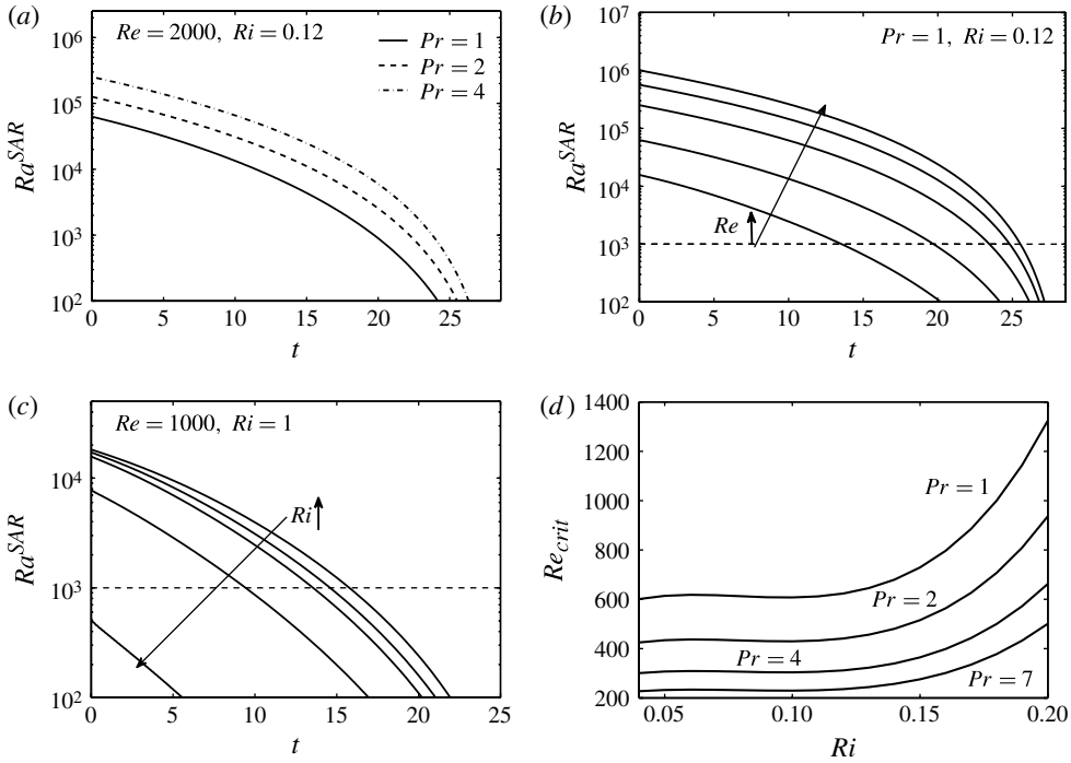
FIGURE 4. (a) Effect of Pr on the Ra'' for Ri_0 = 0.12 and Re = 2000 ; (b) effect of Re on Ra'' for Pr = 1 and Ri_0 = 0.12 ; here Re is increased in the direction of the arrow from 1000 to 2000, 4000, 6000 and 8000; (c) effect of Ri_0 on Ra'' for Pr = 1 and Re = 1000 ; here Ri_0 is increased in the direction of the arrow from 0.04 to 0.08, 0.12, 0.16 and 0.2; (d) critical Re at which Ra'' becomes equal to 1000 at t_m for various Prandtl number values. The horizontal axis in (a–c) represent time elapsed post t_m .
