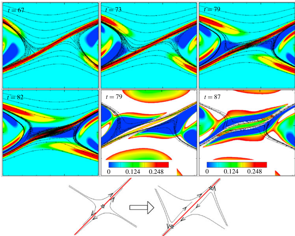
FIGURE 9. The top row and the left panel of the bottom row show the vorticity contours overlaid by the streamlines zoomed on the stagnation point. The contour levels are similar to figure 6. The centre and right figure in the middle row show the contours of the braid Richardson number overlaid by streamlines. Any region with Ri_B > 0.25 is whited out. The final row is a schematic plot which shows the streamlines before and after the core vorticity bands have made the stagnation point to split into two and move further away from the middle of the braid.
