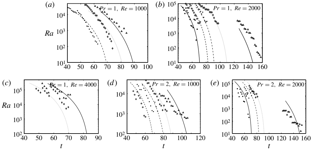
FIGURE 3. Calculations of the Ra^u versus time using the model (lines) plotted alongside data points obtained from the simulations (markers): (a) Pr = 1, Re = 1000 ; (b) Pr = 1, Re = 2000 ; (c) Pr = 1, Re = 4000 ; (d) Pr = 2, Re = 1000 ; (e) Pr = 2, Re = 2000 . The line and marker attributes in each figure are as follows: the solid line with triangles corresponds to Ri = 0.04 , the dotted line with diamonds corresponds to Ri = 0.08 , dashed-dotted line with '+' corresponds to Ri = 0.12 , the dashed line with circles corresponds to Ri = 0.16 and the solid thick line with '*' corresponds to Ri = 0.2 .
