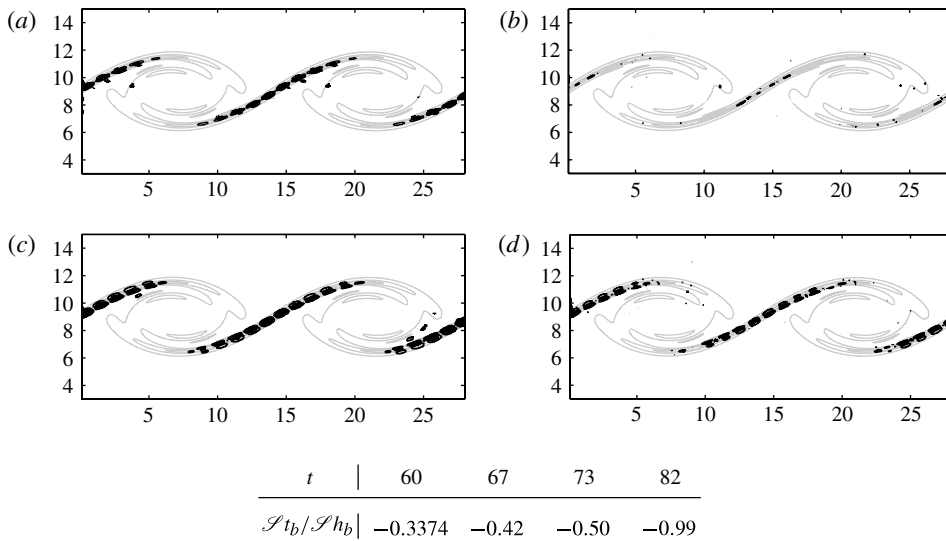
FIGURE 12. Contours of Shear braid eig and Strain braid eig for the SSI of the braid at t = 60 and t = 67 : (a) Shear braid eig contour for SSI at t = 60 , \sigma_r = 1.0 , \mathcal{S}h_b = 1.63 , \mathcal{S}t_b = -0.55 ; (b) Strain braid eig contour for SSI at t = 60 , \sigma_r = 1.0 , \mathcal{S}h_b = 1.63 , \mathcal{S}t_b = -0.55 ; (c) Shear braid eig contour for SSI at t = 67 , \sigma_r = 0.51 , \mathcal{S}h_b = 0.93 , \mathcal{S}t_b = -0.40 ; (d) Strain braid eig contour for SSI at t = 67 , \sigma_r = 0.51 , \mathcal{S}h_b = 0.93 , \mathcal{S}t_b = -0.40 . The table shows the increase with time of the negative relative influence of strain field on the growth of the SSI.
