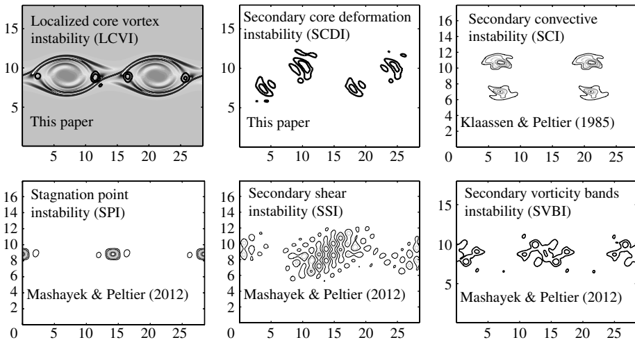
FIGURE 19. Lexicon of various secondary instabilities discussed in this paper and in MP2 . Each frame contains the reference to the original study which provides details of its corresponding instability. The first frame also shows the underlying background KH billow.
