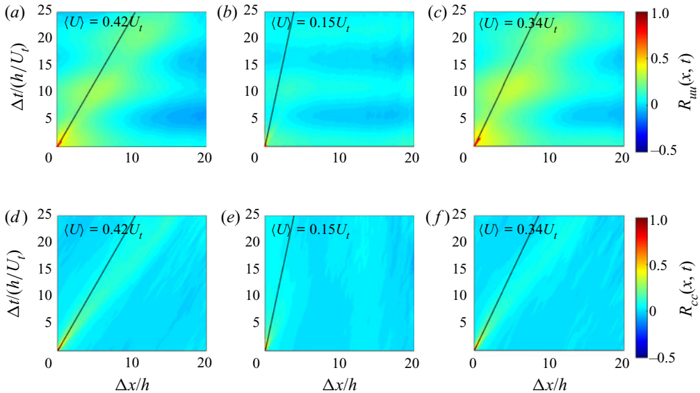
Figure 11. Space–time autocorrelation maps for (a–c) particle velocities and (d–f) concentrations for the case \Phi_V = 2.6 \times 10^{-3} , Re_{bulk} = 1200 . The reference wall-normal distance is (a,d) y/h = 0.2 , (b,e) y/h = 1 and (c,f) y/h = 1.8 . Continuous lines correspond to the local mean velocity, with normalised values indicated in each panel.
