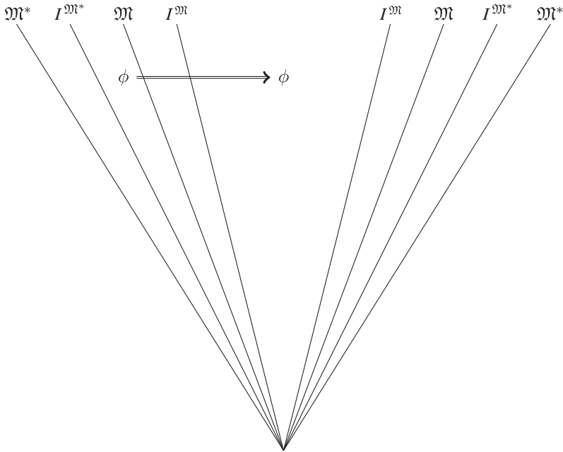
Fig. 1. A visual representation of an application of the \mathfrak{M} -IMH.
