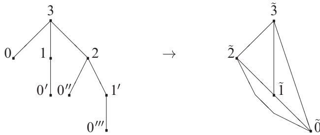
Fig. 6. The quotient process for a coding pair of 3.
