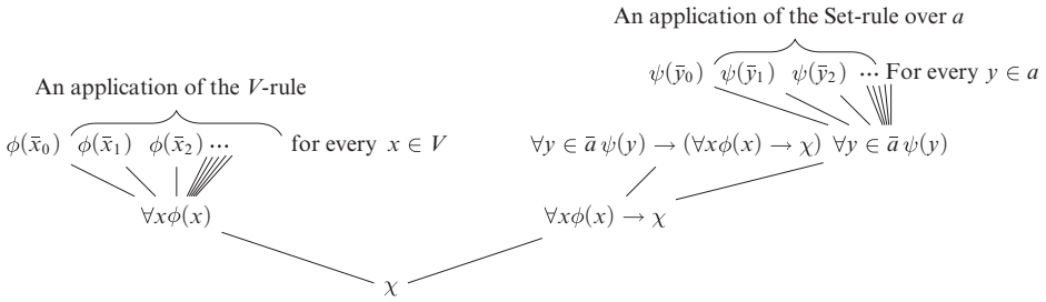
Fig. 3. Visual representation of a proof of \chi in V -logic.
