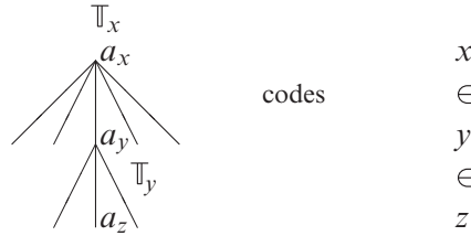
Fig. 4. An example of a tree corresponding to a coding pair showing membership.
