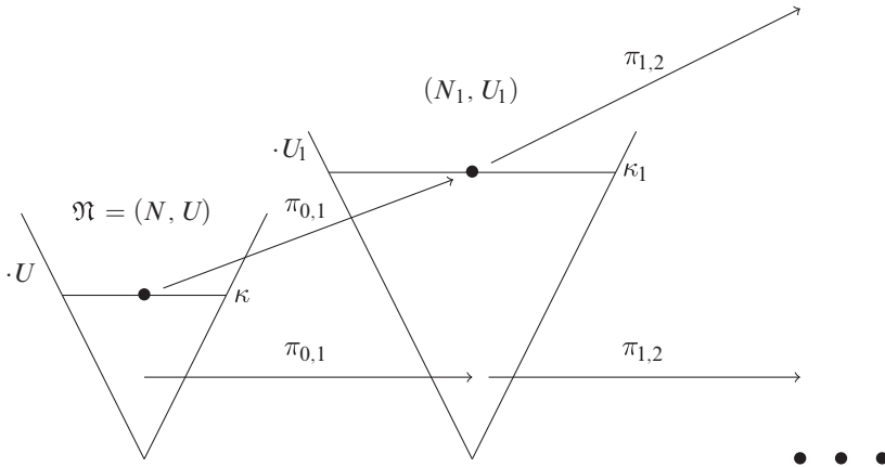
Fig. 2. A visual representation of the initial ultrapowers corresponding to a sharp (N, U) .
