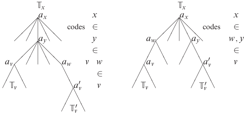
Fig. 5. More complicated coding pair tree structures.
