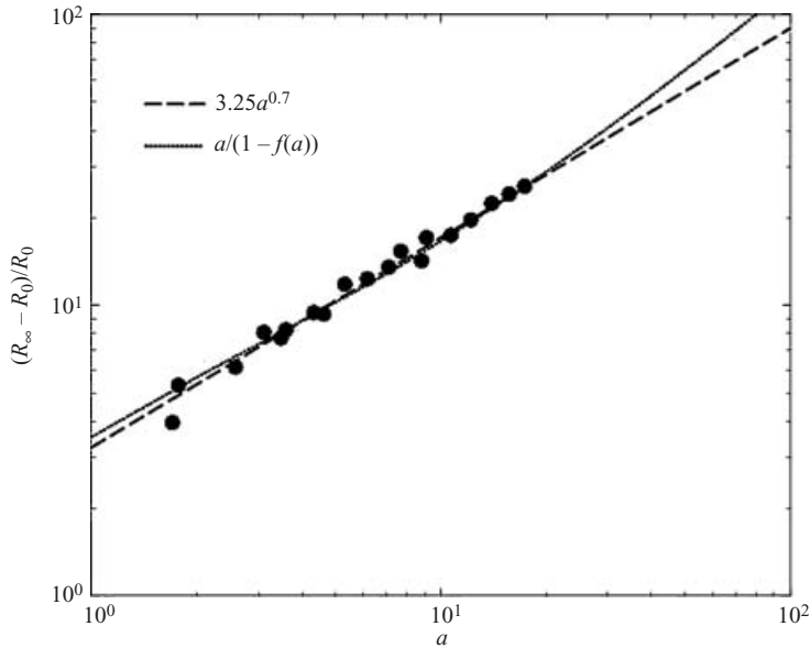
FIGURE 22. Final normalized runout distance (R_\infty - R_0)/R_0 as a function of a . Two different approximations are plotted: the power-law fit in the dashed line, and the function a/(1 - f(a)) in dotted line.
