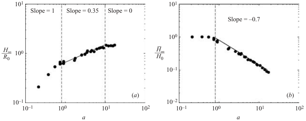
FIGURE 7. Final maximum height of the deposit normalized by the initial radius H_\infty/R_0 (a), and mean height of the final deposit normalized by the initial height \bar{H}_\infty/H_0 (b) as functions of the initial aspect ratio a .
