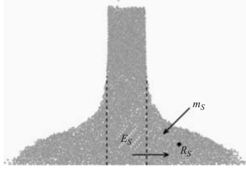
FIGURE 19. During the collapse, the energy E_S and the mass of grains m_S crossing the sections situated at -R_0 and R_0 are evaluated. The centre of mass of the sideways flow is at R_S .
