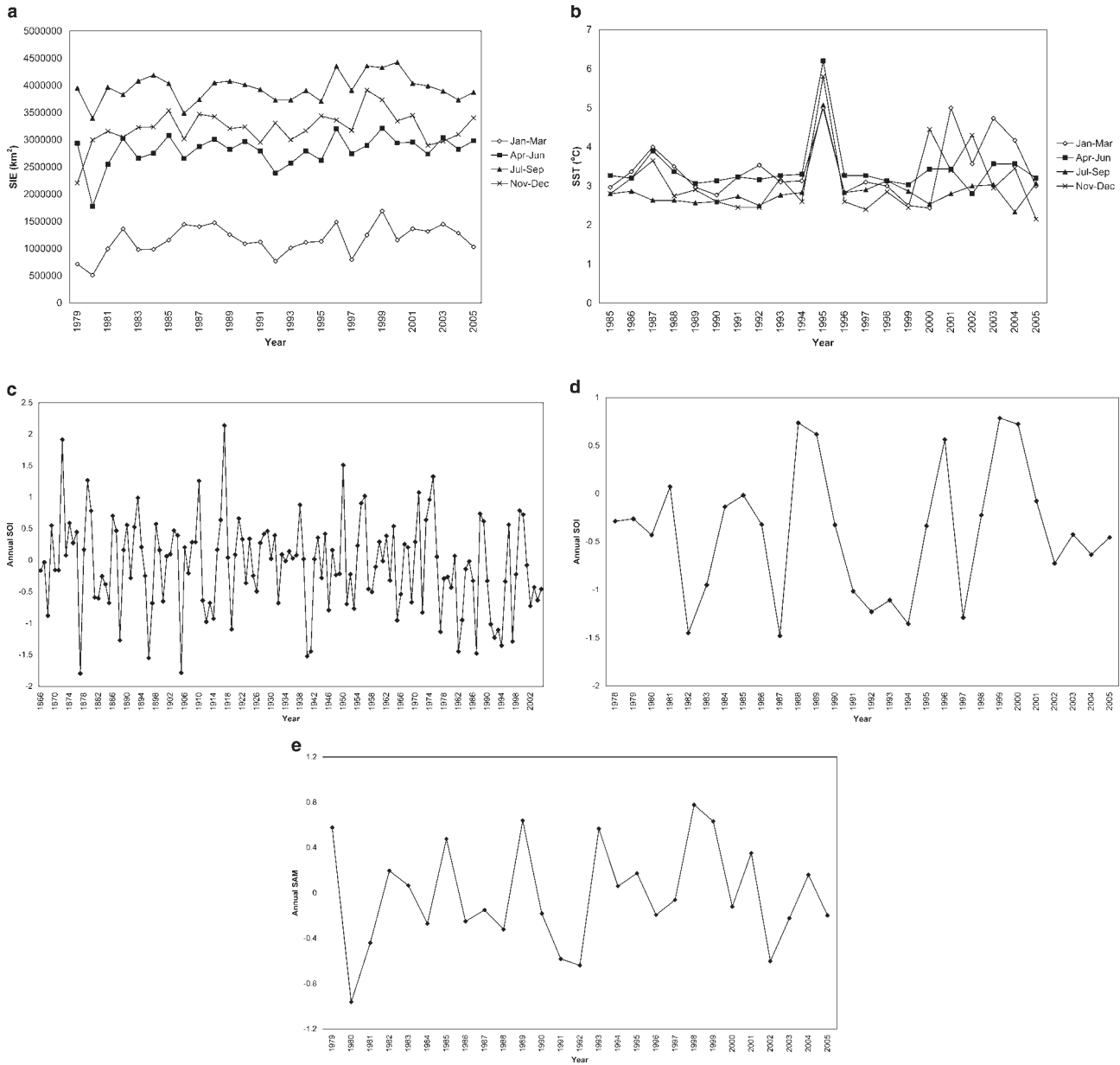
Fig. 2a–e. Sea ice extent (SIE), sea surface temperature (SST), Southern Oscillation Index (SOI), and Southern Hemisphere Annular Mode (SAM) data used in correlations with western Ross Sea emperor penguin live chick counts from 1983–2005.
