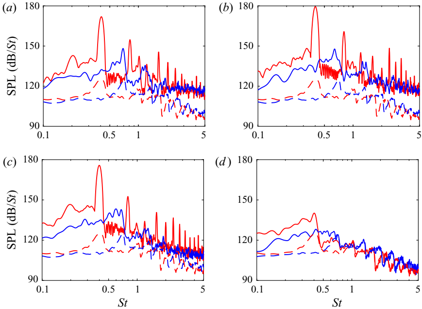
Figure 13. Sound pressure levels (SPL) at z=0 and r=1.5r_0 for (a) jetnohole, (b) jetsmallhole, (c) jetmediumhole, and (d) jetlargehole, for the azimuthal modes for the azimuthal modes n_\theta = 0 (red solid line), n_\theta = 1 (blue solid line) and SPL for the free jet for n_\theta = 0 (red dashed line) and n_\theta = 1 (blue dashed line).
