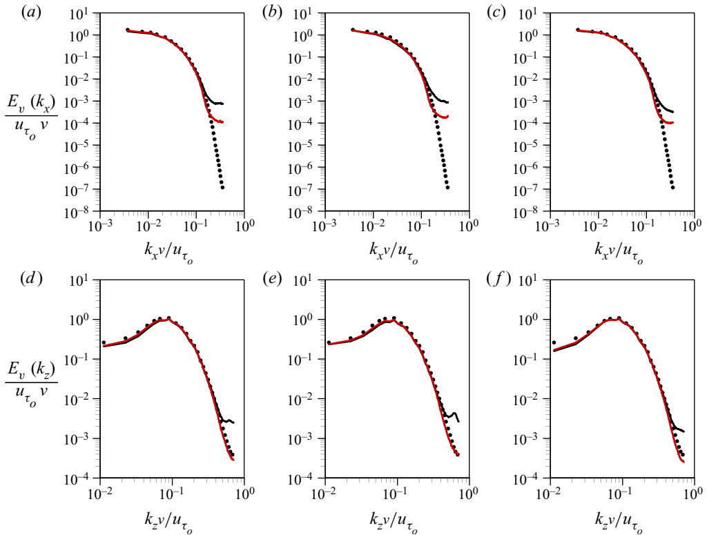
FIGURE 7. Energy spectra of v_{10} from \chi_w = p_w , \partial u/\partial y|_w , and \partial w/\partial y|_w (uncontrolled flow): (a–c) streamwise wavenumber; (d–f) spanwise wavenumber. (a, d) \chi_w = p_w ; (b, e) \chi_w = \partial u/\partial y|_w ; (c, f) \chi_w = \partial w/\partial y|_w . Black circle, v_{10}^{true} (DNS); black line, v_{10}^{pred} with 1P-CNN; red line, v_{10}^{pred} with MP-CNN.
