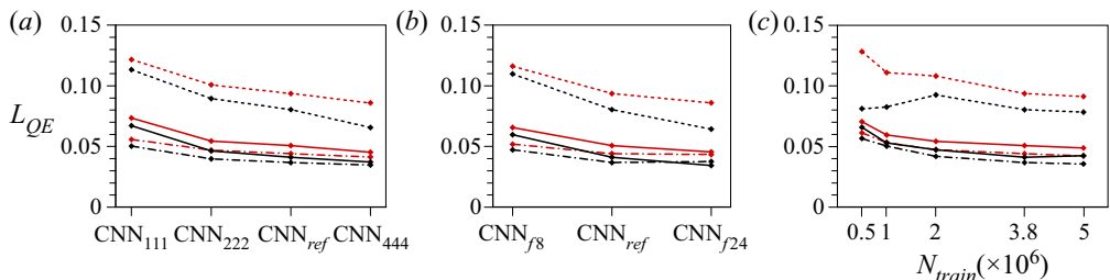
FIGURE 16. Variations of the quadratic error L_{QE} with the parameters used in 1P-CNN: (a) n_1, n_2 and n_3 ; (b) f_m ; (c) N_{train} . —, p_w ; - - - , \partial u/\partial y|_w ; - · - · - , \partial w/\partial y|_w . Black and red lines denote L_{QE} 's for the training and test datasets, respectively.
