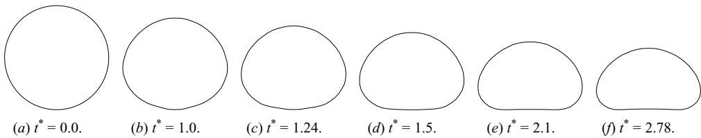
FIGURE 21. Shape of an axisymmetric bubble rising in a tube. The length scale for each of these times is not identical.
