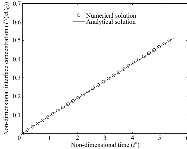
FIGURE 18. Interface concentration as a function of time for an initially clean bubble placed in a bulk medium with uniform initial surfactant concentration. The analytical result is from Muradoglu & Tryggvason (2008).
