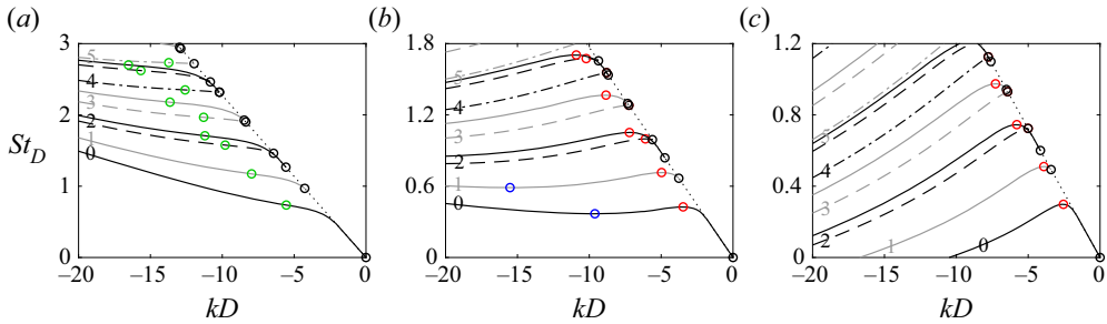
Figure 8. Dispersion relations obtained using the vortex-sheet model for the guided jet waves at (a) M = 0.70 , (b) M = 0.90 and (c) M = 1.10 for n_\theta = 0 (black lines), 1 (grey lines), 2 (black dashed lines), 3 (grey dashed lines), 4 (black dash-dotted lines) and 5 (grey dash-dotted lines) as a function of k and St_D ; points L (black circles), S_{max} (red circles), S_{min} (blue circles) and I (green circles); k = -\omega/c_0 (black dotted lines). For each azimuthal mode, n_\theta is indicated on the dispersion curve for the first radial mode. Only the part with k \leq 0 is shown for M = 1.10 .
