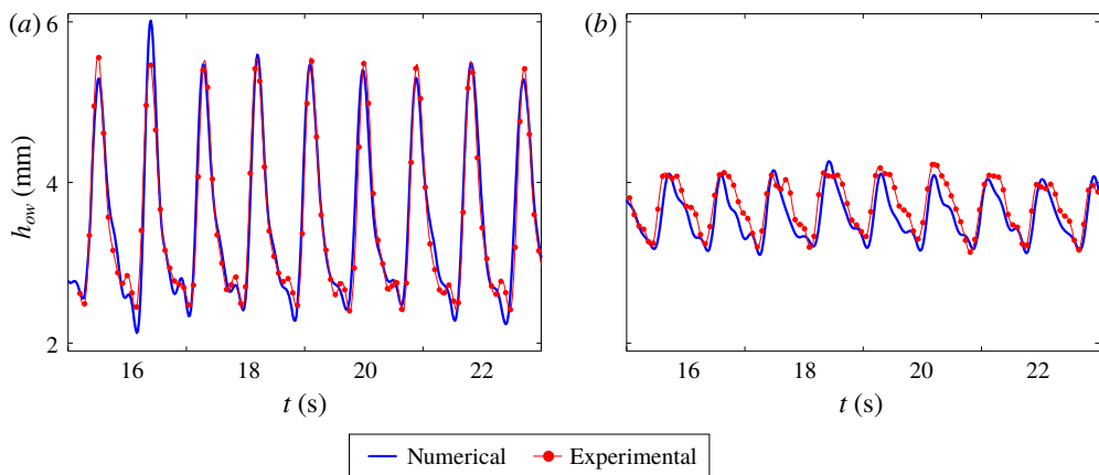
FIGURE 7. Numerical (blue curves) and experimental (red with dots) overshoot depth time series at (a) front end and (b) rear end of the thin plate, with T_{inc} = 0.9 s and ka_{inc} = 0.12 .
