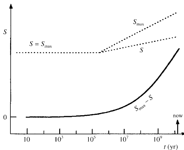
Fig. 4. In the expanding Universe, the actual entropy, S , increases less rapidly than the maximum possible entropy, S_{\max} , once the symmetry of equilibrium broke when matter and radiation decoupled at t \sim 10^5 yr. In contrast, in the early, equilibrated Universe, S = S_{\max} for the prevailing conditions. The potential for the growth of order – operationally defined here as a lack of disorder ( S_{\max} - S ), and shown as the thick black curve – has increased ever since the start of the matter era. Accordingly, the expansion of the Universe can be judged as the ultimate source of free energy, promoting the evolution of everything in the cosmos. This potential rise of order compares well with the curves of Fig. 2 and provides a theoretical basis for the growth of system complexity.
