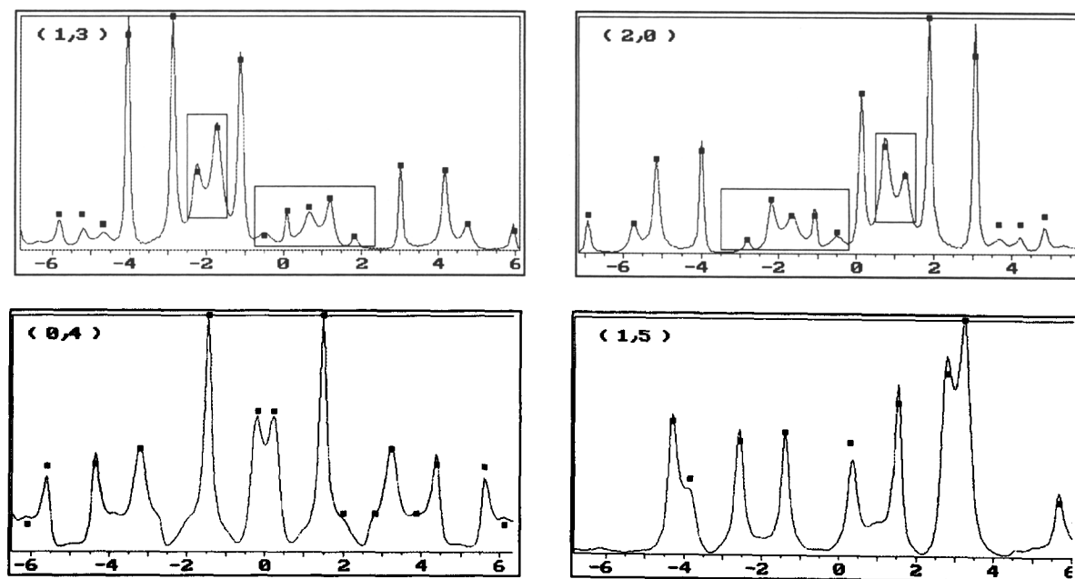
Figure 7. Comparison between experimental and theoretical intensities for the (1, 3), (2, 0), (0, 4) and (1, 5) rods corresponding to the model in which the water is structured in two configurations according to whether it is linked or not to the Mg cation (dots = experimental data).
