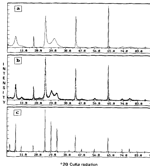
Figure 3. Comparison between the experimental and calculated curves for the (0, 0) rod: a) random interstratification ( W_{Mg} = 0.5 ; P_{Mg/Mg} = 0.5 ); b) the agreement obtained between the experimental and calculated patterns ( W_{Mg} = 0.5 ; P_{Mg/Mg} = 0.7 ); c) regular interstratification ( W_{Mg} = 0.5 ; P_{Mg/Mg} = 1.0 ).
