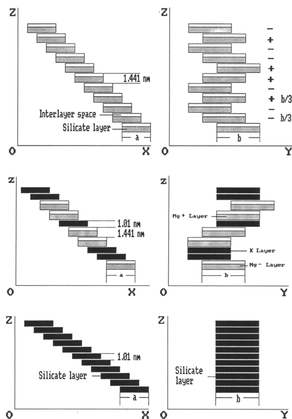
Figure 8. Schematic representation of the stacking modes: Semi-ordered stacking (upper) = two layers of water Mg-vermiculites; intermediate stacking (middle) = mixture of semi-ordered and ordered stacking modes; ordered stacking (lower) = anhydrous K vermiculites.
