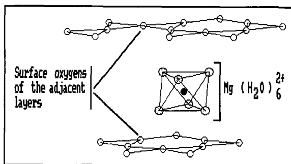
Figure 5. Schematic representation of the interlayer space in a Santa Olalla vermiculite (charge = 0.82, de la Calle et al. , 1988) with a low interlayer water content.
