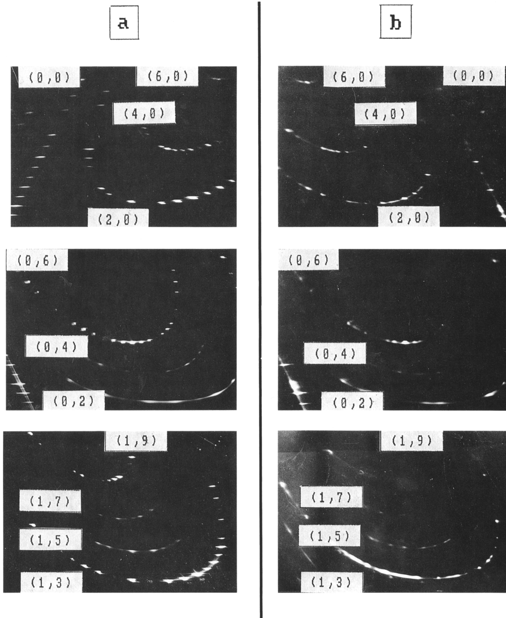
Figure 4. Weissenberg photographs corresponding to the (h, 0) (upper), (0, k) (middle) and (l, k) (lower) rods: a) Mg vermiculite sample before exchange; b) the same sample after treatment with the bi-ionic K/Mg solution = 1/5 at 160°C for 24 hr.
