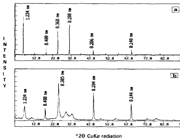
Figure 2. X-ray diffraction patterns along the (0,0) rod: a) Malawi vermiculite before treatment with the bi-ionic K/Mg solutions; b) Malawi vermiculite after treatment with the K/Mg solution = 1/5 at 160°C for 24 hr.
