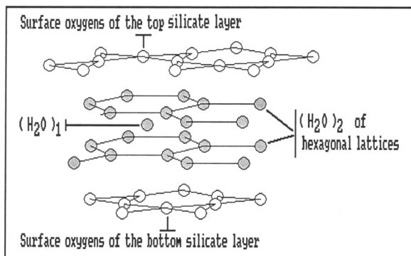
Figure 6. Schematic representation of the configuration of the interlayer "excess" water that is not linked to the Mg cation.
