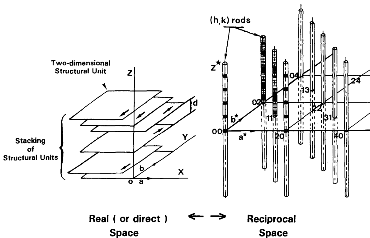
Figure 1. Schematic representation of the reciprocal space corresponding to a semi-ordered stacking mode with \pm b/3 translation faults along Y direction. Note the presence of modulated reciprocal rods (h, k) with k \neq 3n .
