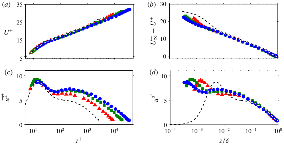
FIGURE 2. (Colour online) Streamwise velocity statistics from the pipe experiments. Panels (a,b) and (c,d) show the mean and variance profiles, respectively. The symbols denote different Re_\tau cases, i.e. \blacktriangle : Re_\tau \approx 10\,000 ( l^+ = 11 ), \blacksquare : Re_\tau \approx 22\,000 ( l^+ = 24 ) and \bullet : Re_\tau \approx 40\,000 ( l^+ = 44 ), while the dashed (---) lines correspond to the statistics from Ahn et al. (2015) at Re_\tau \approx 3000 ( 2\pi R^+/N_\theta = 6 , where N_\theta is the number of grids in the DNS along the azimuthal direction).
