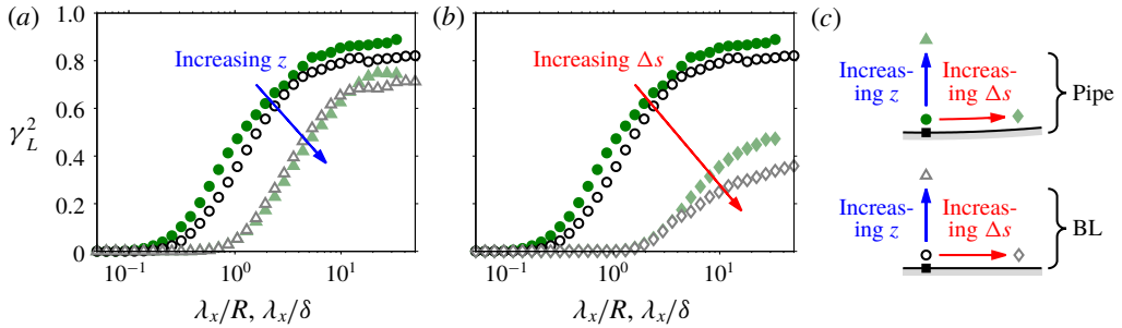
FIGURE 7. (Colour online) Coherence spectrum, \gamma_L^2 , between the streamwise velocity, u , and the friction velocity, u_\tau , as a function of wavelength \lambda_x . The solid ( \bullet , \blacktriangle , \blacklozenge ) and open ( \circ , \triangle , \diamond ) symbols respectively correspond to the pipe and boundary layer (BL) flows. Also, the pipe and boundary layer flows are at Re_\tau \approx 22\,000 and 14\,000 , respectively. (a) Two wall heights z/R, z/\delta \approx 0.01 ( \bullet , \circ ) and 0.07 ( \blacktriangle , \triangle ) at \Delta s \approx 0 ; and (b) two hot-film offsets \Delta s/R, \Delta s/\delta \approx 0 ( \bullet , \circ ) and 0.07 ( \blacklozenge , \diamond ) at z/R, z/\delta \approx 0.01 are shown. (c) Schematic of hot-wire and hot-film positions used to generate (a) and (b), where \blacksquare symbol denotes the reference skin friction sensor.
