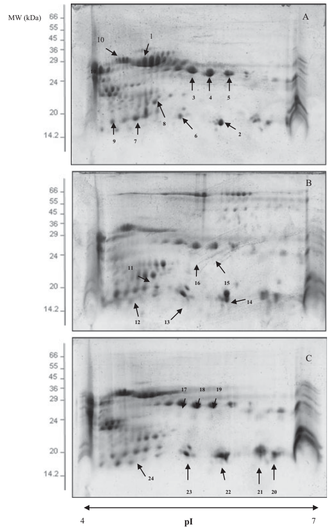
Fig. 3. Two-dimensional gel electrophoretograms of cheeses made in April (a), August (b) or December (c) separated under reducing conditions using a 7 cm pH 4–7 pI range for the first dimension and a 12% gradient acrylamide SDS-PAGE gel for the second dimension.
