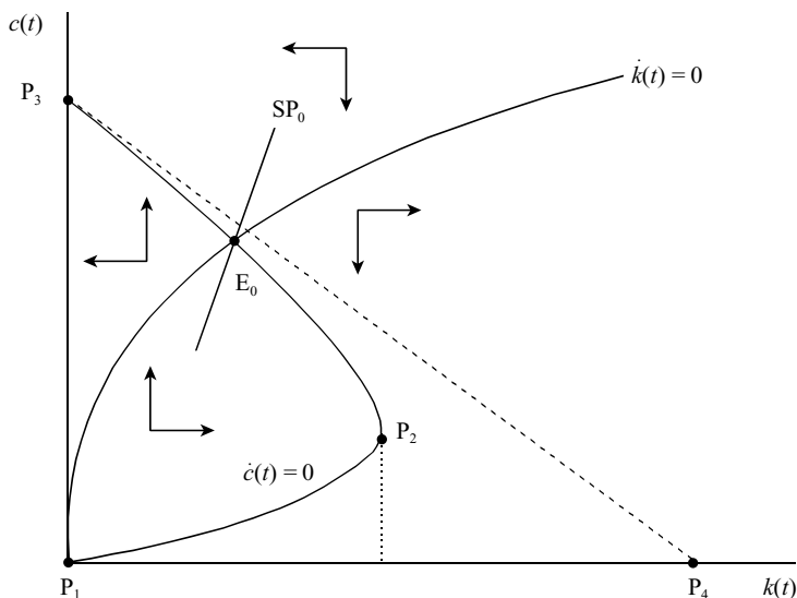
FIGURE 1. Phase diagram.
