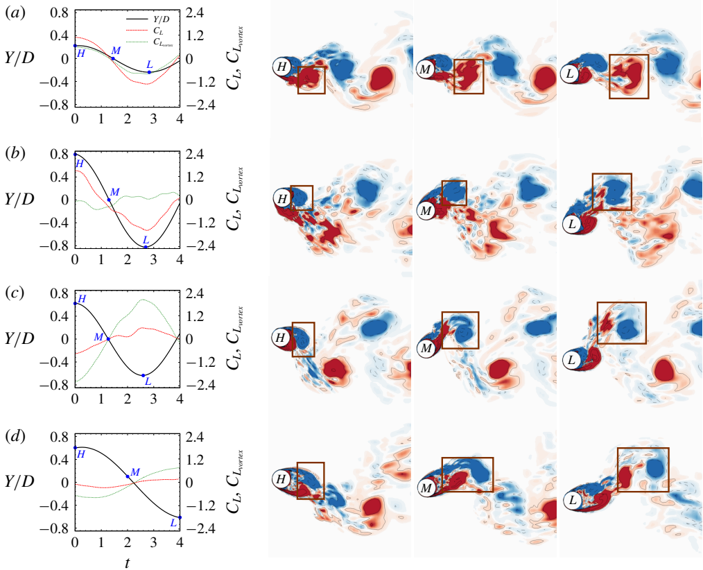
FIGURE 5. Flow past a freely vibrating cylinder for (a) U^* = 4.7 ( IB response), (b) U^* = 5.3 ( UB^* response during intermittency), (c) U^* = 5.3 ( LB^* response during intermittency) and (d) U^* = 8.0 ( LB response). The line plot shows the time histories of the cylinder transverse displacement, C_L and C_{L_{vortex}} as the cylinder descends from its highest to lowest transverse location, while the remaining columns show the instantaneous span-averaged spanwise vorticity near the highest ( H ), mean ( M ) and lowest ( L ) transverse position of the cylinder. These locations as well as the corresponding time instants are marked on the curve for transverse displacement in the line plot. For each case, a certain flow structure is tracked via a rectangular frame.
