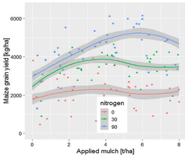
Fig. 4. Interaction effects of residue biomass levels and N fertilizer on grain yield at University of Zimbabwe site in 2014 growing season.
