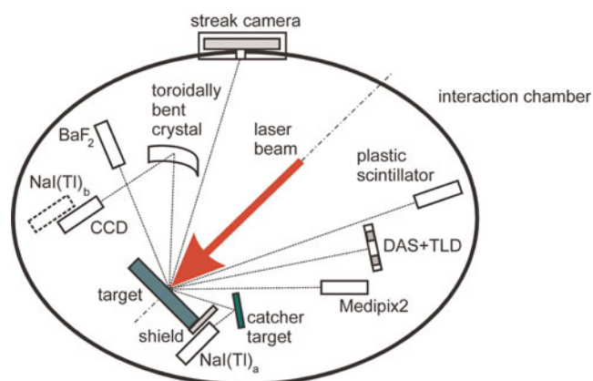
Fig. 3. (Color online) Scheme of the experimental setup.
