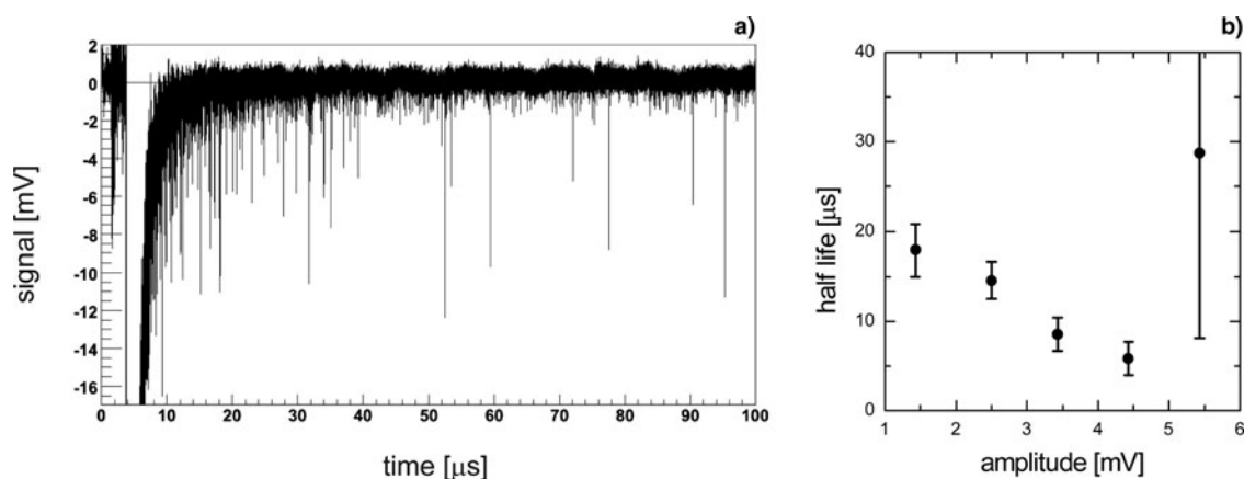
Fig. 6. Analysis of typical signals detected by the BaF 2 scintillator (a) provides ambiguous amplitude dependent alternatives for determination of the decay half-life (b).
