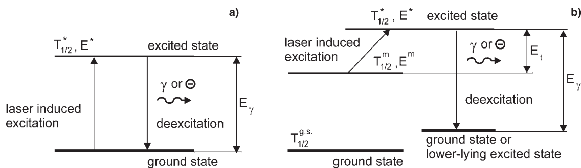
Fig. 2. Excitation and decay in stable and long-lived unstable nuclei (a) and isomers (b).
