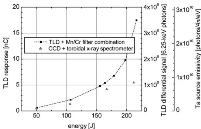
Fig. 5. Absolutely calibrated Ta plasma emissive centered at 6.25 keV. A dashed line connects points measured with the absorption foils method, scatter points were obtained with the crystal spectrometer.
