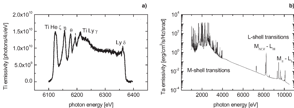
Fig. 4. Emission spectrum of the H- and He-like Ti ions used for calibration of the spectrometer (a) and the Ta spectrum synthesized by the FLYCHK code (b).
