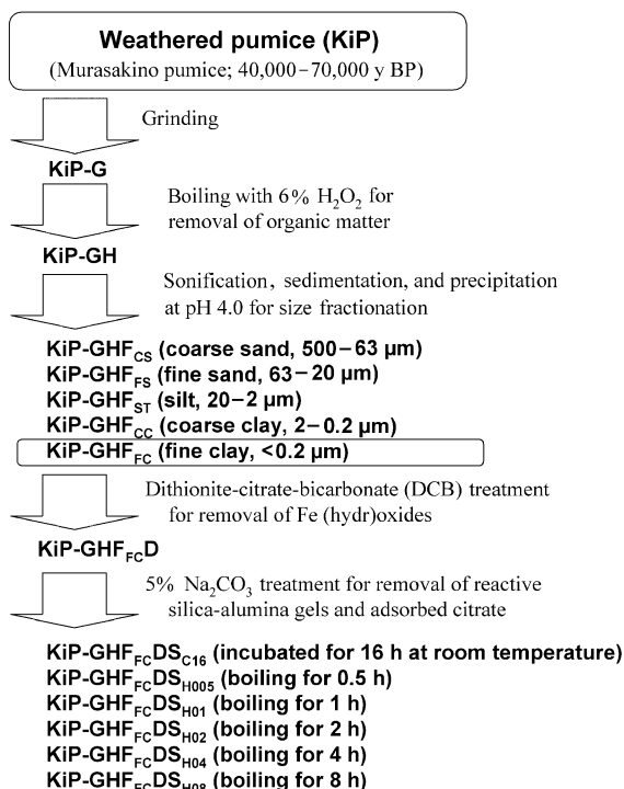
Figure 1. Purification procedure of allophane from weathered pumice (Murasakino pumice; 40,000–70,000 y BP).
