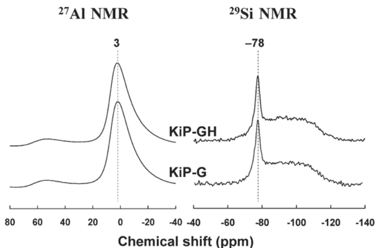
Figure 2. Solid-state ^{27}\text{Al} and ^{29}\text{Si} NMR spectra of untreated (KiP-G) and 6% \text{H}_2\text{O}_2 -treated (KiP-GH) ground pumice.
