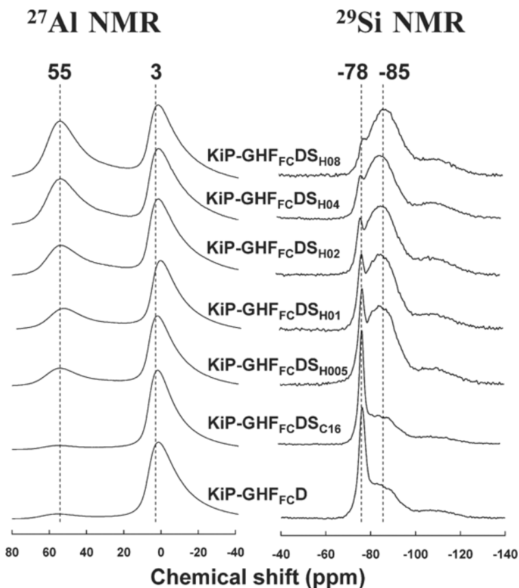
Figure 5. Influence of 5% \text{Na}_2\text{CO}_3 treatment on solid-state ^{27}\text{Al} and ^{29}\text{Si} NMR spectra of allophane. KiP-GHF FC D; untreated control, KiP-GHF FC DS C16 ; incubated for 16 h at room temperature, KiP-GHF FC DS H005 ; boiling for 0.5 h, KiP-GHF FC DS H01 ; boiling for 1 h, KiP-GHF FC DS H02 ; boiling for 2 h, KiP-GHF FC DS H04 ; boiling for 4 h, KiP-GHF FC DS H08 ; boiling for 8 h.
