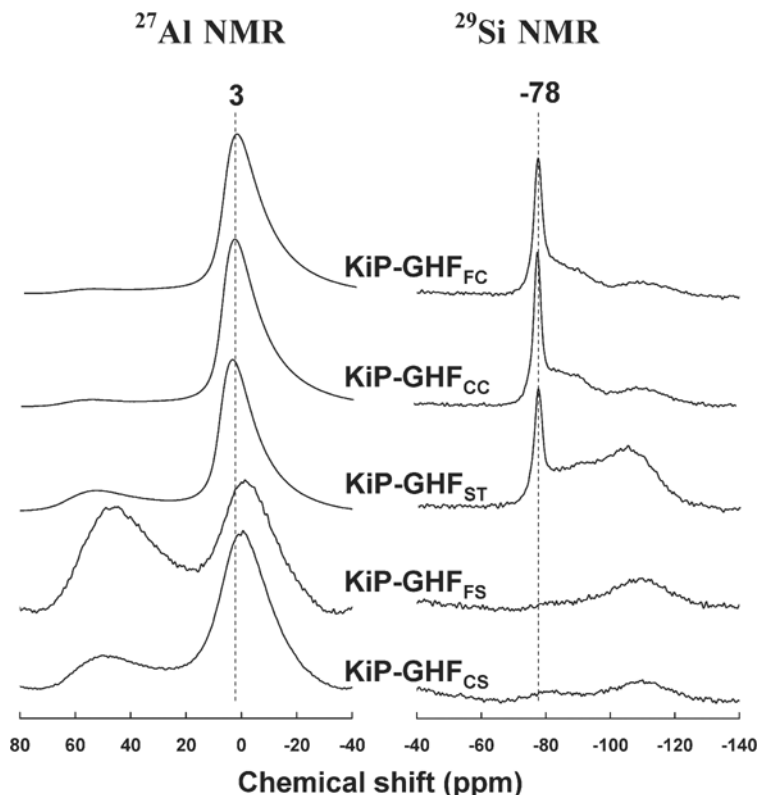
Figure 3. Solid-state ^{27}\text{Al} and ^{29}\text{Si} NMR spectra of coarse sand (KiP-GHF CS ; 500–63 \mu\text{m} ), fine sand (KiP-GHF FS ; 63–20 \mu\text{m} ), silt (KiP-GHF ST ; 20–2 \mu\text{m} ), coarse clay (KiP-GHF CC ; 2–0.2 \mu\text{m} ), and fine clay (KiP-GHF FC ; <0.2 \mu\text{m} ) fractions of the \text{H}_2\text{O}_2 -treated ground pumice (KiP-GH).
