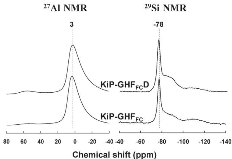
Figure 4. Comparison of solid-state ^{27}\text{Al} and ^{29}\text{Si} NMR spectra between before-(KiP-GHF FC ) and after-(KiP-GHF FC D) dithionite-citrate-bicarbonate treatment of the fine clay fraction of the \text{H}_2\text{O}_2 -treated ground pumice.
