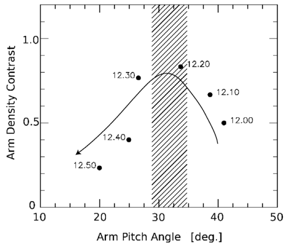
Figure 10. Evolution of spiral arm on \alpha - \bar{\delta} plane for T_{rot} = 12.0 - 12.5 . The hatched region corresponds to the predicted maximum pitch angle around the analysed region ( Q \approx 1.4 and \Gamma \approx 0.8 ) due to swing amplification (refer to Equation (98) in Fuchs (2001)). From Baba et al. (2013).
