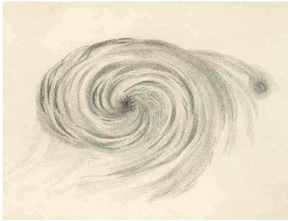
Figure 1. A sketch of M51 by Lord Rosse (Rosse 1850).
