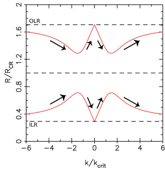
Figure 3. Propagation diagram for tight-winding stellar density waves following the LSK dispersion relation (Equation 8). The disc is assumed to have a flat rotation curve and constant Toomre's Q = 1.2 . The horizontal dashed lines are the OLR radius (upper), CR radius (middle), and ILR radius (lower), respectively. The arrows indicate the directions of group velocities. Long waves ( |k/k_{crit}| \ll 1 ) are reflected at the Lindblad resonances, while short waves ( |k/k_{crit}| \gg 1 ) are absorbed there due to Landau damping.
