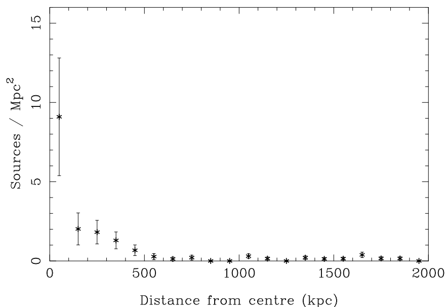
Figure 4 —Radial distribution of identified radio galaxies selected from 23 D \leq 4 clusters on the basis of their absolute magnitudes (see Section 6). The Abell radius is R_A = 2000 kpc.
