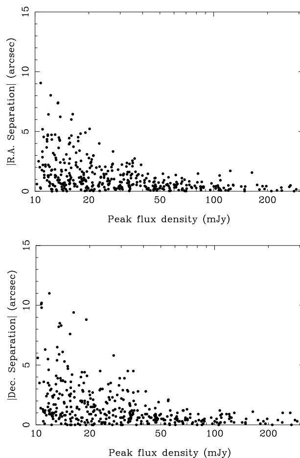
Figure 1 —Differences in RA (top) and Dec (bottom) between pairs of observations of identical sources (after subtraction of systematic offsets and removal of obvious outliers), as a function of peak flux density. The variances in RA and Dec differences were fitted to equation (1) to define the noise component of position uncertainties.
