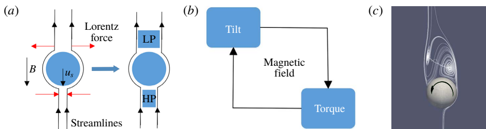
FIGURE 4. (Colour online) Understanding the transition onset of a horizontal velocity. (a) A compact model for the influence of the magnetic field. ‘HP’ and ‘LP’ stand for ‘high pressure’ and ‘low pressure’, respectively, due to the Lorentz force. The high pressure in the HP region pushes away the streamlines and the Lorentz force in the LP region directly pulls away the streamlines. (b) A positive feedback effect for the fluid–solid system. (c) Three-dimensional streamlines projected onto the symmetric plane at Re = 250 with N = 0 in a fixed sphere case.
