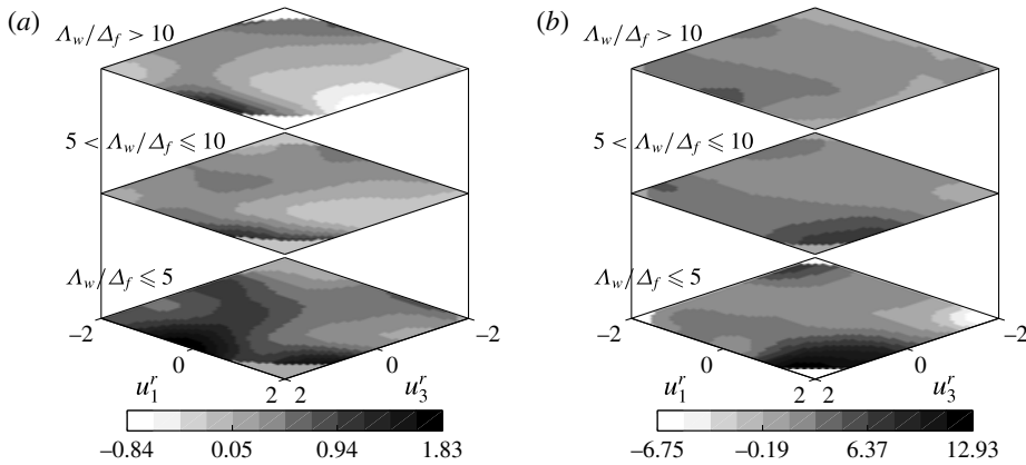
FIGURE 10. Conditional mean SGS pressure transport of \langle \tau_{33} | \mathbf{u}^r \rangle , \langle \partial T_{333}^{(p)} / \partial x_3 | u_1^r, u_3^r \rangle , for the (a) weakly convective ( 0 < -z/L \leq 0.3 , with mean -z/L = 0.23 ) and (b) strongly convective ( 1 < -z/L \leq 2.5 , with mean -z/L = 1.83 ) surface layers.
