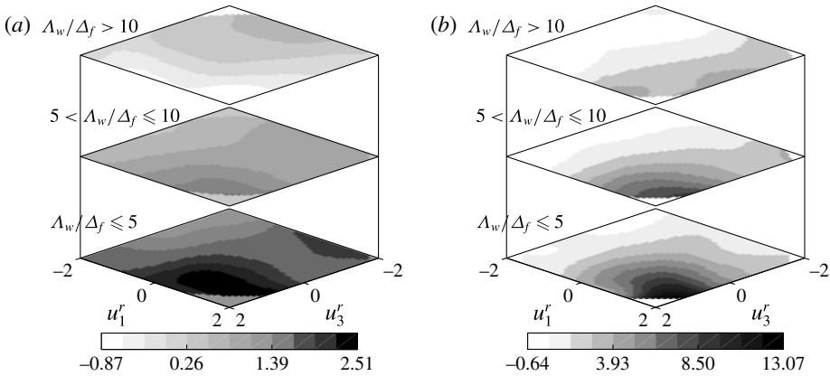
FIGURE 14. Conditional mean SGS velocity–pressure-gradient correlation in the transport equation of \langle \tau_{13} | \mathbf{u}^r \rangle , \langle \Pi_{13} | u_1^r, u_3^r \rangle , for the (a) weakly convective ( 0 < -z/L \leq 0.75 , with mean -z/L = 0.23 ) and (b) strongly convective ( 1.75 < -z/L \leq 2.5 , with mean -z/L = 1.83 ) surface layers.
