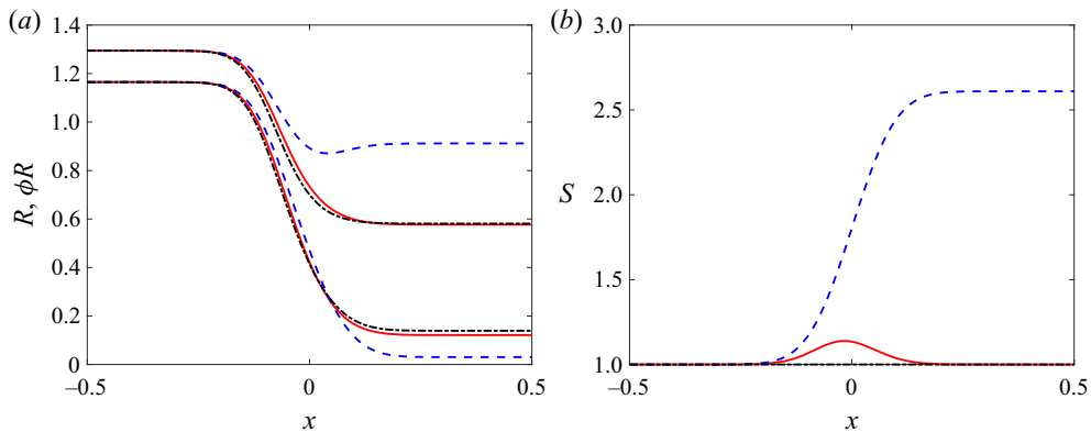
FIGURE 4. Geometry (a) R and \phi R and (b) cross-sectional area S versus axial position x for the 1-D (black dash-dot), 2DT+ (red solid) and 2DT0 (blue dashed) models with \beta = 9 and V = 1.6 . For the 1-D model S(x) = 1 .
