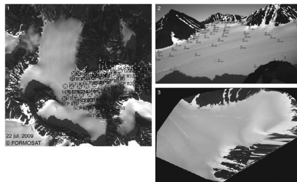
Fig. 5. 1: Map of the reference points used for the geometric correction for camera number 3. All the points on the glacier surface are 2m \times 2m flags located using a Coarse/Acquisition (C/A) code GPS, while reference points of the slopes and ridges are visually identified. 2. Each point is paired with a set of pixel identified on one reference picture of each camera, here camera number 3 in the naming convention of Fig. 1. 3. Resulting geometrically corrected image. All processing performed on the images acquired on 22 July 2009.
