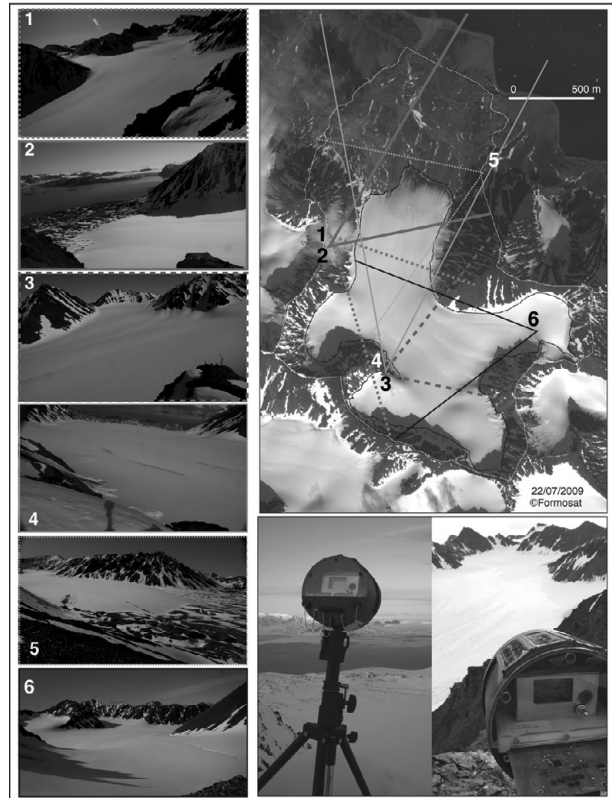
Fig. 2. Positioning of the 6 cameras used to monitor the glacier (the other cameras installed on the glacier basin focus on the moraine), with the field of view of each camera and a typical image captured by each instrument on a sunny day. Bottom right: experimental setup, in which a COTS digital camera is packaged in a waterproof, air tight enclosure. Solar panels complement the lithium batteries for powering the on-board real time clock used for providing the date of each image in the EXIF header.
